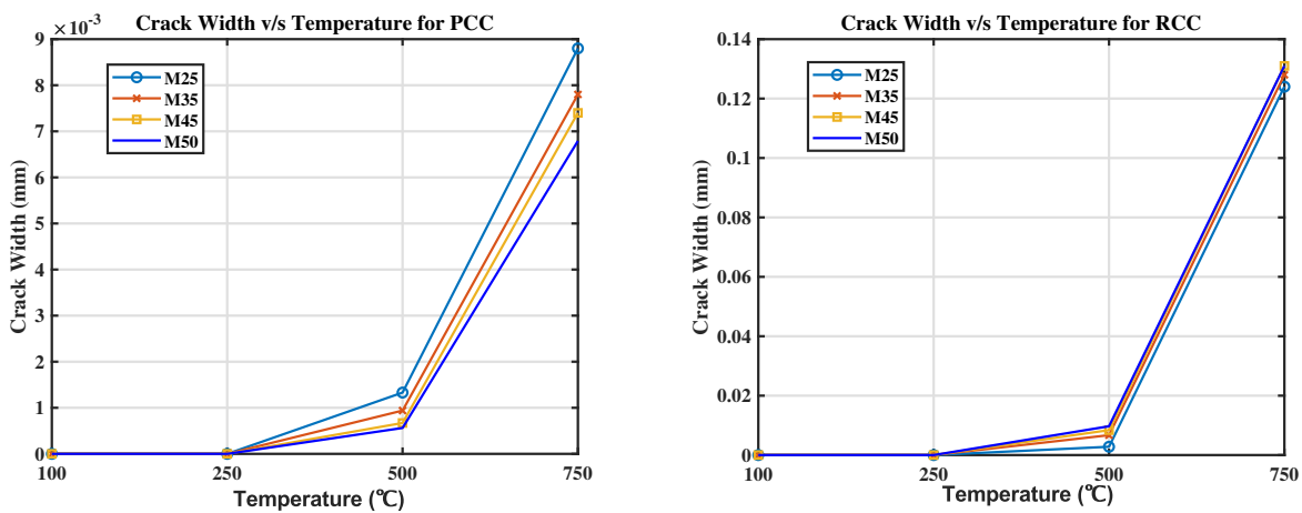
Figure 9: Crack width for both concrete type at different temperatures
