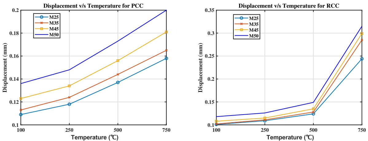
Figure 7: Variation in Displacement with temperature for PCC and RCC
