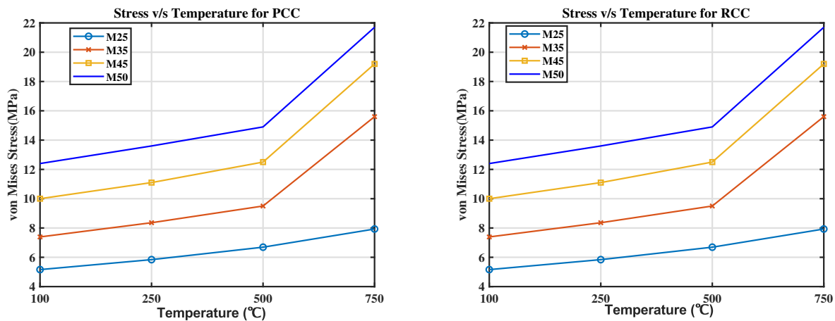
Figure 11: von Mises stress comparison of PCC and RCC for different grades with temperature
