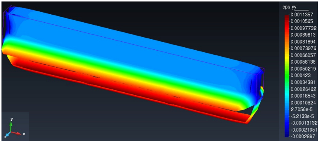
Figure 13: FEM model representation of strain for RC-M45 at 750 ^{\circ}\text{C}
