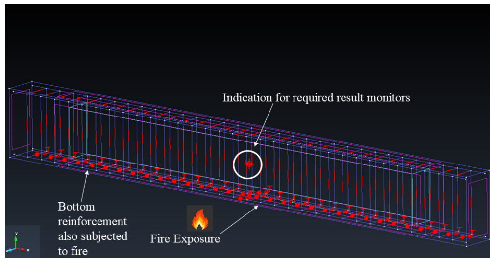
Figure 3: External loading conditions where bottom surface of beam and bottom reinforcement is exposed to fire
