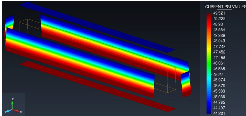
Figure 6: FEM model representation of thermal results for RC-M35 at 500°C
