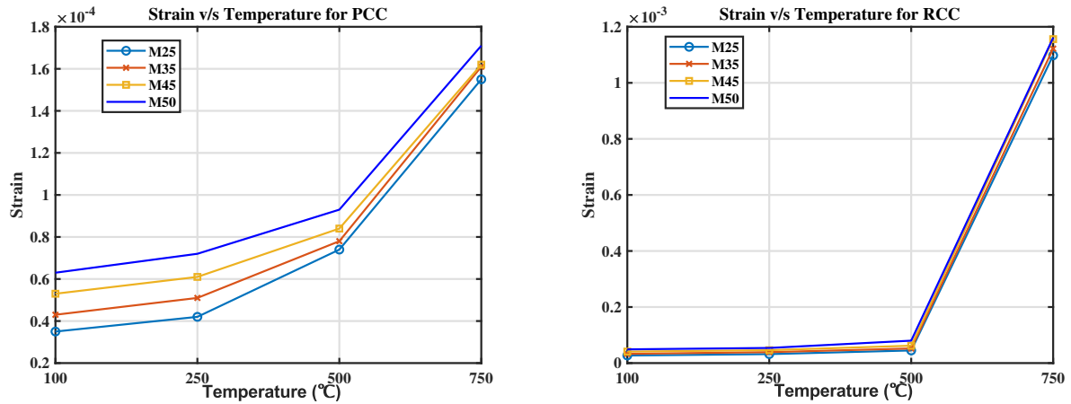
Figure 12: Strain variation with temperature for PCC and RCC
