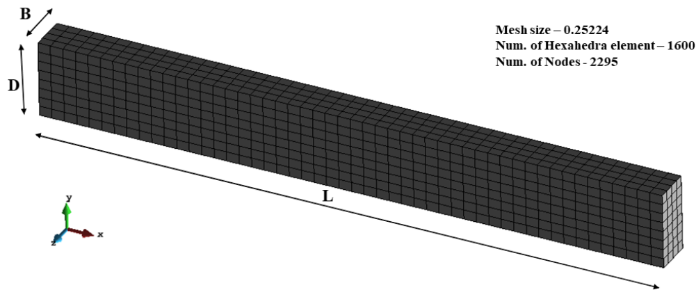
Figure 2: ATENA beam model with mesh representation
