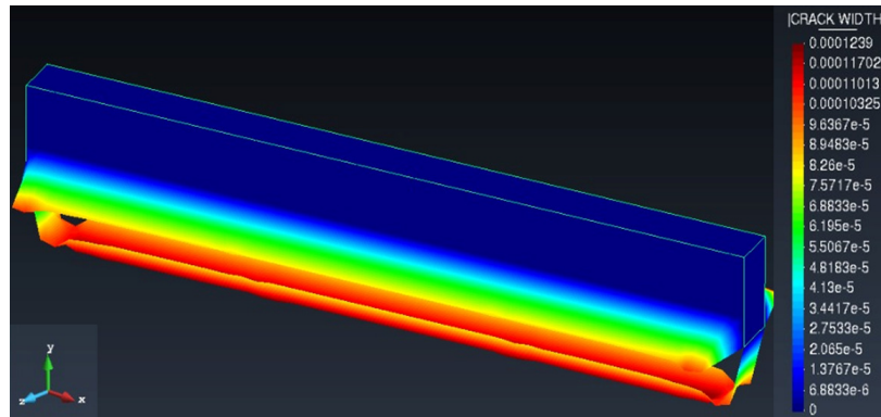
Figure 10: FEM model representation of crack width for RC-M25 at 750°C
