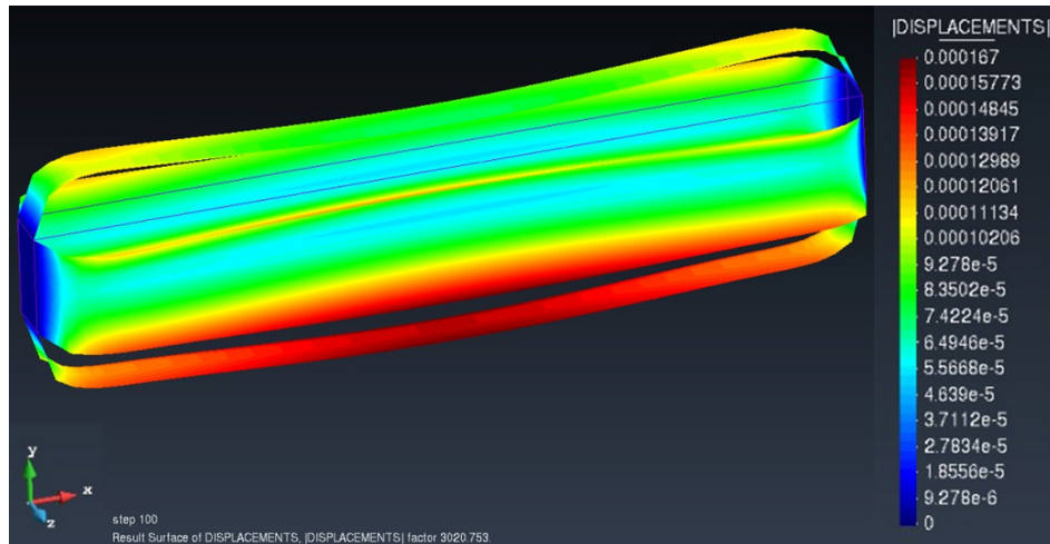
Figure 8: FEM model representation of displacement for PC-M45 at 750°C
