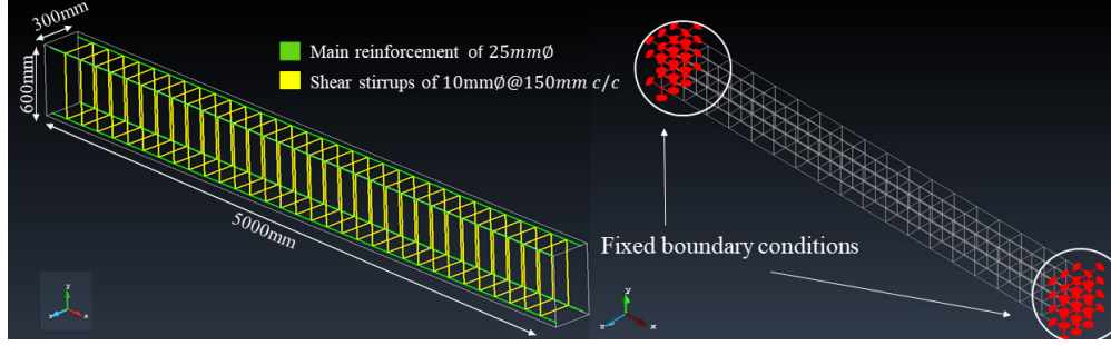
Figure 1: ATENA beam model with reinforcement details (left) and boundary conditions (right)
