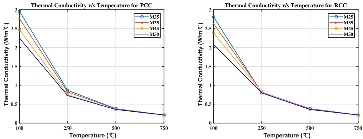
Figure 5: Thermal conductivity for PCC and RCC with temperature
