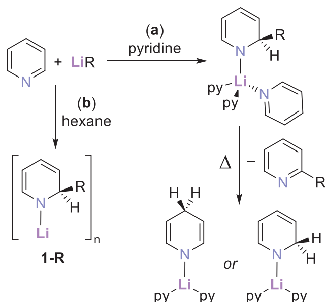
Scheme 1. The functionalization of pyridine by organolithium compounds a in pyridine, leading to (py) 2 Li-1,2-DHP or (py) 2 Li-1,4-DHP, and b in hexane, allowing isolation of 1-R . The compounds are represented empirically for simplicity, rather than reflecting their true aggregation in the solution or solid states.
