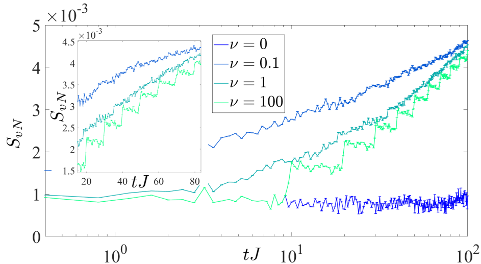
Figure 5: Entanglement Entropy and dependence on noise space heterogeneity. S_{vN} vs time tJ in a log scale for different levels of collision-time homogeneity \nu and fixed low collision rate r_c = 0.1 , large disorder range h = 10 and anisotropy \Delta = 2.5 in the interesting plateaus regime, for a disordered spin chain of N = 20 sites and two injected excitations starting next to each other. Inset: same in the main figure, but in linear scale. The plot shows the mean S_{vN} over 25 of the total M = 250 trajectories.
