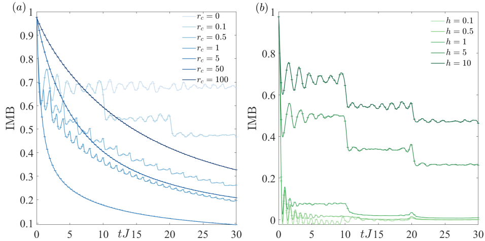
Figure 6: Imbalance for the One excitation case. (a) Imbalance for a spin chain of N = 41 sites and N_{exc} = 1 excitations starting in the middle of the chain, shape parameter \nu = 100 , disorder range constant h = 10 and interaction strength \Delta = 0 for different collision rates. Final time is tJ = 30 . (b) Imbalance versus time for a spin chain of N = 41 sites, one excitation, different disorder range constants at fixed collision rate r_c = 0.1 , shape parameter \nu = 100 and anisotropy \Delta = 0 . The simulations were performed with M = 500 trajectories and dt = 0.02 .
