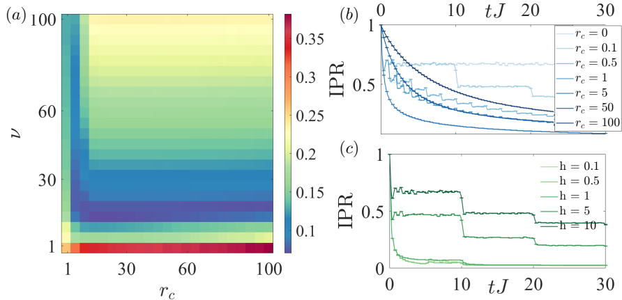
Figure 2: (De)localization behaviour: one excitation case. Inverse Participation Ratio (IPR) for a spin chain with N = 41 sites. (a) IPR at long time ( tJ = 30 ), for h = 10 and different shape parameters \nu and collision rates r_c . (b) IPR vs time for large disorder range h = 10 for different collision rates r_c . (c) IPR vs time tJ for low r_c = 0.1 and different disorder range h . Notice the emergence of plateaus of temporary stabilization of localized behavior. For (b) and (c) the shape parameter is \nu = 100 in the time-homogeneous collision regime. The data refer to the case of no anisotropy ( \Delta = 0 in Eq. 1) since they are seen to be not significantly altered by finite \Delta \neq 0 . The simulations were performed with M = 500 trajectories and dt = 0.02 .
