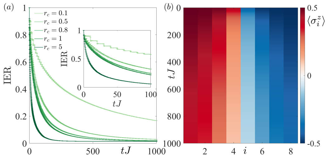
Figure 4: Case of multiple excitations. Inverse Ergodicity Ratio (IER) (a) and color plot of the magnetization (b) for a spin chain of N = 8 sites and N_{exc} = 4 excitations starting in the middle sites, time-homogeneous collisions \nu = 100 , with high disorder range width h = 10 and anisotropy strength \Delta = 2.5 . (a) IER vs time tJ for different collision rates r_c in the interesting regime as in the legend. (b) Spread of magnetization over time tJ and sites i in the interesting regime of low collision rates, here e.g. with r_c = 0.1 . We can overall see that low collision rates ( r_c \ll 1 ) combined with time-homogeneous collisions ( \nu = 100 ) lead the system to remain localized for a significant time, prolonged also by the presence of anisotropy and high disorder. Only at very long times the IER approaches its asymptotic value, signaling full delocalization. The simulations were performed with M = 250 trajectories and dt = 0.02 . Final time is tJ = 1000 .
