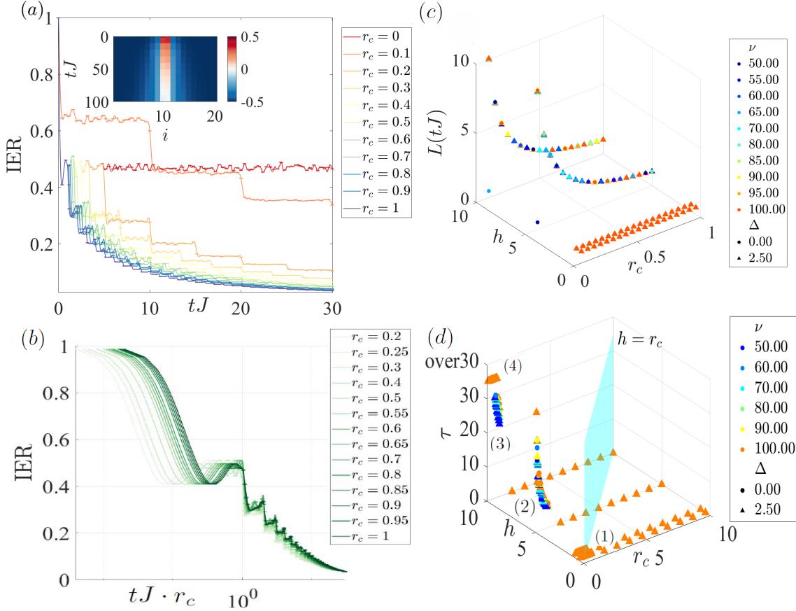
Figure 3: Effect of anisotropy: the case of two excitations. Inverse Ergodicity ratio (IER) with associated magnetization, plateau length and delocalization time \tau for a spin chain of N = 20 sites and final time of simulations tJ = 30 . (a) IER vs time tJ for different collision rates r_c with anisotropy strength \Delta = 2.5 . Inset: magnetization map over sites i and time tJ , showing the spreading of the two excitations over time. The two neighbouring excitations are initially separated by two spins with very homogeneous collisions over time ( \nu = 100 ) and high disorder range with h = 10 . The IER has the same trend of the IPR and we focus here on the collision rate regime 0 \leq r_c \leq 1 , proved to be more interesting due to the formation of plateaus. For lower collision rates ( r_c \ll 1 ) the systems remains localized (IER closer to 1), while increasing r_c leads to a faster delocalization (IER decaying to its limit). (b) IER vs tJ r_c varying the collision rate parameter 0 \leq r_c \leq 1 , at fixed high time-homogeneity ( \nu = 100 ), high disorder strength ( h = 10 ), and in the presence of anisotropy, considering two excitations initially separated by two spins.
