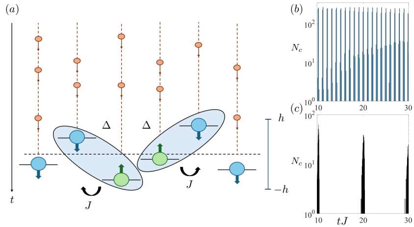
Figure 1: Sketch of our model. (a) Open quantum spin chain with energy levels affected by disorder in the [-h, h] range. Excitations are depicted as flipped spins (green), their dynamics being affected by the tunneling rate J (black arrows), interaction strength \Delta (blue ovals) and the addition of a noisy environment. This is represented by the auxiliary light-brown qubits colliding with the sites over time. (b)-(c) Histograms displaying the number of collisions undergone by the auxiliary qubits (log scale) against our spins over time tJ for a noise shape parameter of \nu = 100 in the time-uniform regime, and collision rates r_c = 1 (b) and (c) r_c = 0.1 . We use the same simulation parameter: number of sites in the spin is N = 41 sites, M = 500 trajectories and final time of simulation tJ = 30 .
