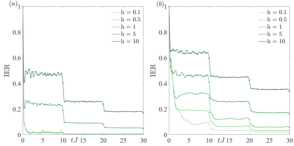
Figure 7: Two excitations case. Inverse Ergodicity ratio (IER) for a spin chain of N = 20 sites and final time of simulations tJ = 30 . (a) IER vs time tJ for different disorder range constants at fixed r_c = 0.1 , \nu = 100 , \Delta = 2.5 for two excitations starting initially separated by two spins and (b) two excitations starting next to each other. The simulations were performed with M = 250 trajectories and dt = 0.02 .
