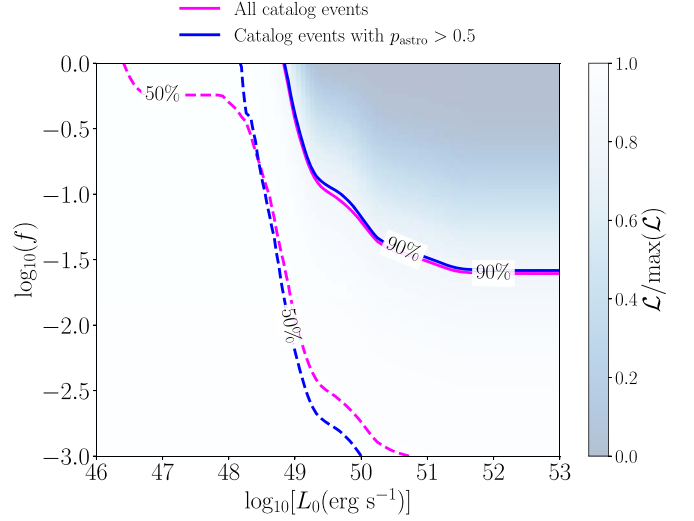
Figure 7. Constraints on the two parameters L_0 and f of the model for the putative EM counterpart of BBH mergers. The color map reports the likelihood \mathcal{L}_i for the full analysis including all the O3 catalog events with p_{\text{astro}} > 0.5 . L_0 is in units of \text{erg s}^{-1} . The thick blue solid and dashed contours indicate the exclusion regions in the [L_0, f] plane at 90% and 50% credibility levels, respectively. The magenta solid and dashed lines report the same contours, but for an analysis that includes all O3 catalog events, with no cut in p_{\text{astro}} .
