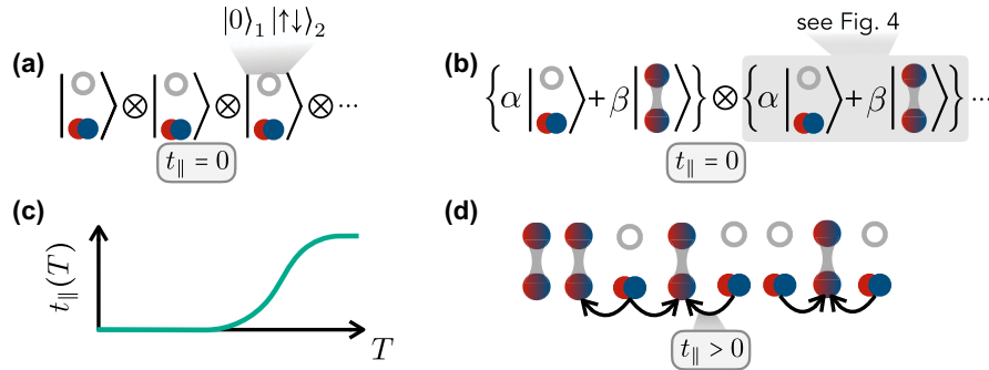
FIG. 5. State-preparation scheme. State preparation for simulating the mixD t - J model on a ladder. (a) A band insulating state is prepared in deep double wells with \Delta > U . (b) Tuning \Delta = U for a given amount of time, singlets are created with a certain average density |\beta|^2 (where still t_{||} = 0 ), cf. Fig. 4. Afterwards, \Delta is tuned to \Delta < U . (c) Hopping between double wells is adiabatically turned on by ramping down the lattice potentials, which enables the simulation of the mixD bilayer model on a ladder geometry in step (d).
