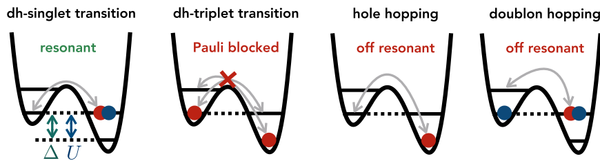
FIG. 7. Allowed and blocked transitions. Applying a \pi/2 pulse by tuning \Delta = U leads to the following effect depending on the local configuration: transitions between local rung singlets and doublon-hole pairs are resonant. Meanwhile, transitions between local rung triplets and doublon-hole pairs are Pauli-blocked and interlayer hopping of single holes and doublons is off resonant.
