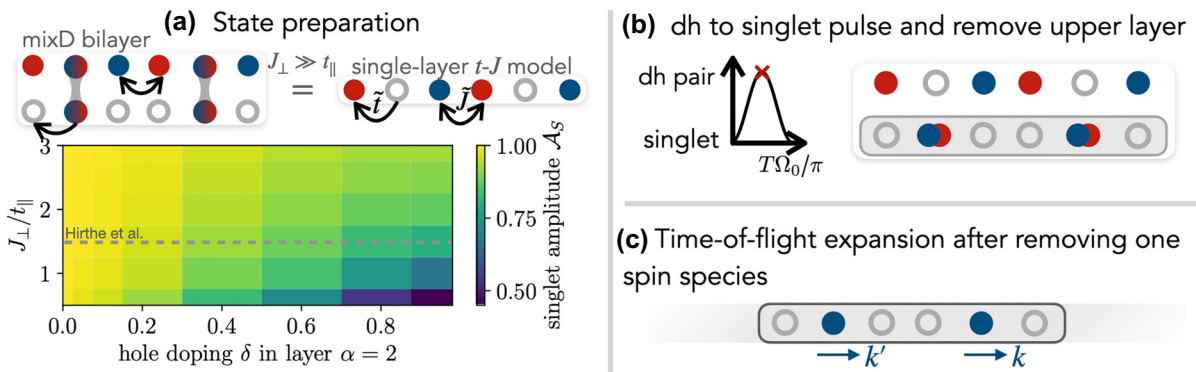
FIG. 9. Measurement protocol of momentum-resolved density. (a) State preparation. For large J_\perp/t_\parallel , singlets form on the rungs of the mixD layer and allow the system to be mapped to a 2D single-layer t - J model. We also show numerical results for the rung-singlet probability \mathcal{A}_S [see Eq. (40)] obtained for a ladder of length L = 40 and different hole dopings of the lower leg \delta (i.e., hole doping 1 - \delta of the effective t - J model). We use J_\perp/t_\parallel and J_\parallel/t_\parallel = 0.07 as used in Hirthe et al. [41]. After the state preparation, a \pi -basis rotation is applied (b), which maps all singlets to dh pairs with doublons in the lower \alpha = 2 layer and holes in the upper \alpha = 1 layer. When removing one spin species from the lower layer and ramping down the lattice depth (c), the remaining indistinguishable particles—one per dopant—are free and their momentum can be measured using a time-of-flight protocol.
