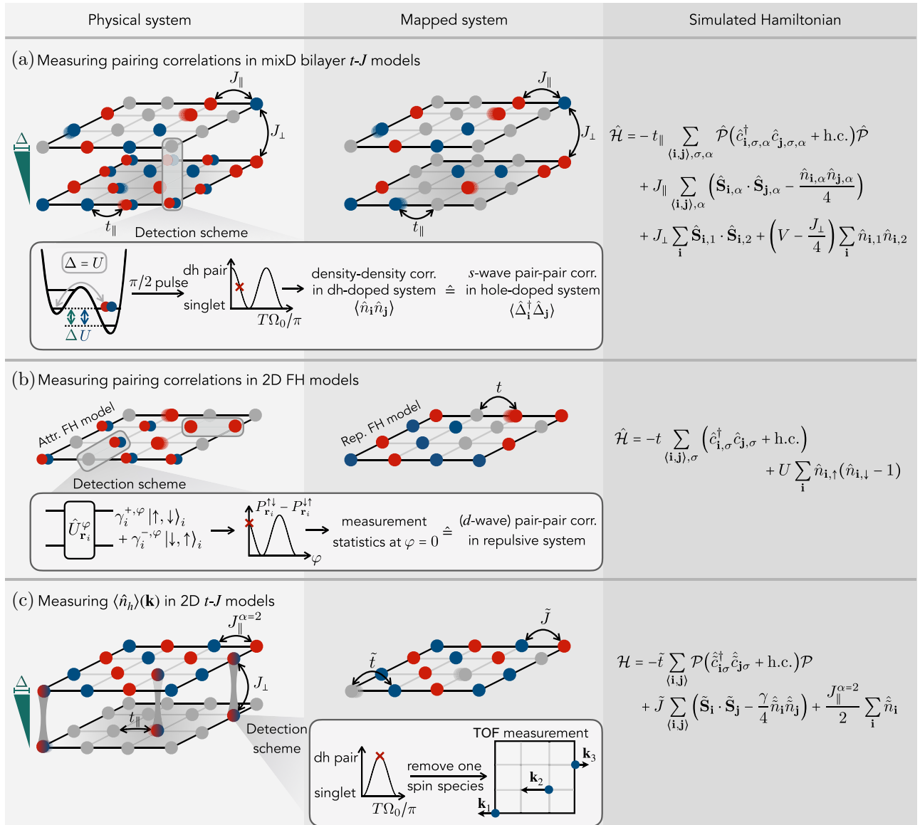
FIG. 1. Exploring high-temperature superconductivity with optical lattices. (a) Scheme showing how to measure coherent pairing correlations in the mixD bilayer t - J model. We propose to implement the Fermi-Hubbard model in the strong-coupling limit on a bilayer geometry (physical system). By applying a potential gradient \Delta between the two layers, interlayer tunneling is suppressed, such that t_{\perp} = 0 , but J_{\perp} > 0 . Up to tunable interlayer density-density interactions, the model relates to a fully hole-doped mixD bilayer t - J model through a partial particle-hole transformation (mapped system). In the physical, doublon-hole-doped system, performing a global resonant tunneling pulse ( \Delta = U ) after ramping up the lattice depth results in Rabi oscillations with frequency \Omega_0 between singlets and doublon-hole (dh) pairs on the rungs. In a \pi/2 rotated basis (red cross), density-density correlations in the doublon-hole-doped system then correspond to coherent pair-pair correlations in the fully hole-doped system. The protocol is described in Sec. II. (b) In a similar spirit, the 2D repulsive FH model relates to its attractive counterpart by a partial particle-hole transformation. To measure pairing correlations of various symmetries (including d wave) \langle \hat{\Delta}_{\mathbf{r}_1}^\dagger \hat{\Delta}_{\mathbf{r}_2} \rangle between bonds \mathbf{r}_1 and \mathbf{r}_2 , we propose to implement the attractive FH model and apply local gates with unitaries \hat{U}_{r_i}^\varphi acting on bonds \mathbf{r}_i . This gives rise to a Ramsey interferometer as a function of a controlled phase dependency \varphi , from which pairing correlations can be accessed in the repulsive model. In particular, probabilities P_{r_i}^{\sigma_1 \sigma_2} of measuring |\uparrow, \downarrow\rangle and |\downarrow, \uparrow\rangle states after applying the local gates correspond to pairing correlations in the repulsive model. The protocol is described in Sec. III (c) By preparing the upper layer of a mixD setup at half-filling and loading (particle) dopants into the (initially empty) lower layer, singlets can be mapped to holes in an effective 2D t - J model for J_{\perp} \gg t_{\parallel}, J_{\parallel}^{\alpha=1,2} . Singlet-to-dh transitions then give access to momentum-resolved hole densities via time-of-flight measurements in the lower layer. The protocol is described in Sec. IV.
