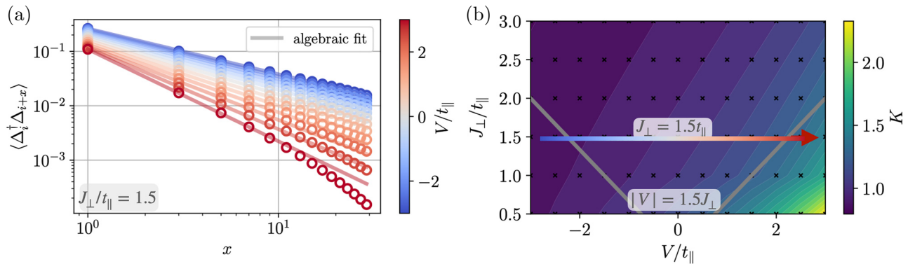
FIG. 3. DMRG simulations. (a) Coherent pairing correlations \langle \hat{\Delta}_i^\dagger \hat{\Delta}_{i+x} \rangle in the ground state of a mixD ladder of length L_x = 60 at hole doping \delta = 0.5 , for experimentally relevant couplings J_\parallel/t_\parallel = 0.5 and J_\perp/t_\parallel = 1.5 [41] and for various interaction strengths V/t_\parallel . Fits to algebraic decay functions are shown by solid lines; for illustrative reasons, only odd distances are shown. (b) Luttinger decay exponents K as a function of J_\perp/t_\parallel and V/t_\parallel . Contours denote extrapolated lines of constant K , black dots the points evaluated for the extrapolation. The arrow with the color gradient indicates the V/t_\parallel scan in (a) from attractive (blue) to repulsive (red) interactions. Gray lines show typical interaction strengths for \Delta = U/2 , V = 1.5J_\perp , see Eq. (16).
