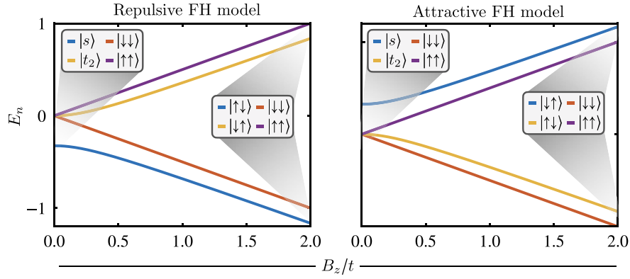
FIG. 11. Adiabatic magnetic field gradient ramp. Evolution of instantaneous eigenstate energies of Hamiltonian Eq. (A8) as a function of B_z/t , with U/t = 12 ( U/t = -12 ) on the left-hand (right-hand) side. For B_z/t = 0 , triplet states are degenerate and energetically offset from the singlet state. While |\uparrow\uparrow\rangle and |\downarrow\downarrow\rangle stay invariant under the adiabatic transformation, the singlet state transforms to |\uparrow\downarrow\rangle ( |\downarrow\uparrow\rangle ), and the triplet state to |\downarrow\uparrow\rangle ( |\uparrow\downarrow\rangle ) in the repulsive (attractive) case. This allows (i) a singlet to be distinguished from triplet states in spin-resolved snapshots, as required in the measurement scheme, Sec. II E, and (ii) the transformation |\uparrow\downarrow\rangle \rightarrow |t_2\rangle to be applied through a reversed adiabatic protocol as proposed in the measurement scheme, Sec. III C.
