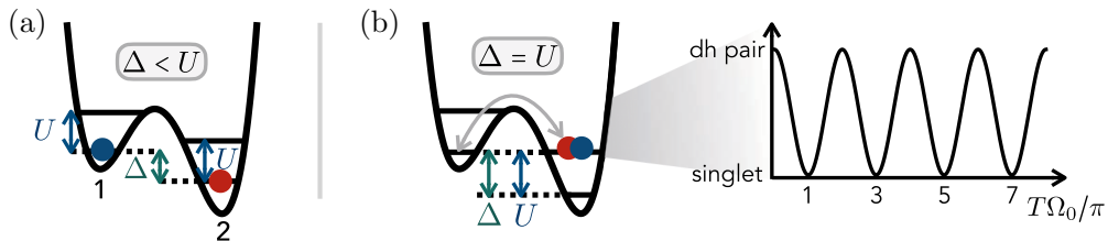
FIG. 4. Double-well Rabi oscillations. (a) A single double-well building block with energy shift \Delta < U . The ground state with one particle per site is a singlet state. (b) When tuning \Delta = U to resonance, coherent Rabi oscillations (in time T ) between singlets and doublon-hole pairs are induced, with holes (doublons) situated in the energetically upper (lower) site, labeled site 1 (2).
