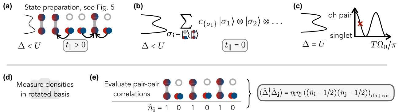
FIG. 6. Measurement protocol. After state preparation [cf. Fig. 5] in step (a), lattice potentials are ramped up to freeze out t_\parallel = 0 , (b). A \pi/2 basis rotation by tuning U = \Delta (c) and consecutively measuring densities of singlets and doublon-hole pairs (d) then allows for evaluation of pair-pair correlations in step (e).
