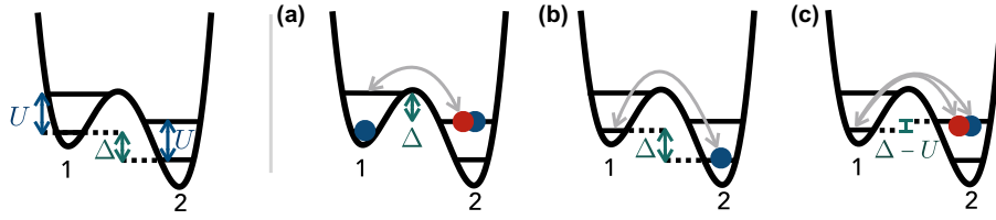
FIG. 2. Interlayer interactions. Left panel: illustration of the double-well geometry with on-site interaction U and energy offset \Delta ; here, layer 1 (2) is the energetically upper (lower) layer. In the doublon-hole-doped setting, virtual processes lead to the appearance of nearest-neighbor interlayer interactions between particles. Contributions come from (a) a particle in the upper ( \alpha = 1 ) and a doublon in the lower ( \alpha = 2 ) layer, (b) a hole in the upper and a particle in the lower layer, and (c) a hole in the upper and a doublon in the lower layer.
