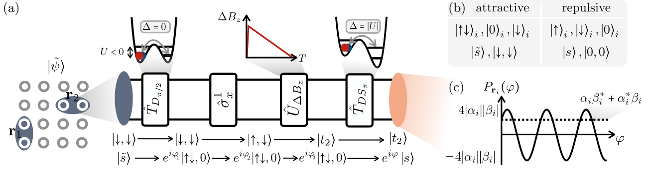
FIG. 8. Measuring pairing correlations in the plain-vanilla FH model. (a) Circuit that allows measurement of coherent pair-pair correlations in the repulsive FH model between bonds \mathbf{r}_1, \mathbf{r}_2 through implementation of the attractive FH model. The mapping from the attractive to the repulsive side is summarized in (b). The shown sequence in (a) consists of a combination of local tunneling and spin gates. The former are realized by locally reducing the lattice depth and tuning the superlattice offset \Delta . Adiabatic tuning of a magnetic field gradient \Delta B_z allows |\downarrow, \downarrow\rangle to be mapped [corresponding to the hole-pair state in the repulsive model, see (b)] to a spin-triplet, whereas |\tilde{s}\rangle [corresponding to |s\rangle in the repulsive model, see (b)] is transformed to a spin singlet. After each step, relative phases between the two input states are picked up, with an overall phase shift of \varphi between the end of the sequence. Spin-resolved measurements after applying the unitary allow for the evaluation of pairing correlations P_{ij}^{\alpha, \beta} in the repulsive FH model. (c) The overall phase difference \varphi between the final output states gives rise to oscillations of measurement probabilities P_{r_i} , from which \langle (\hat{\Delta}_{\mathbf{r}_1}^\dagger + \hat{\Delta}_{\mathbf{r}_1}) (\hat{\Delta}_{\mathbf{r}_2}^\dagger + \hat{\Delta}_{\mathbf{r}_2}) \rangle = (\alpha_1 \beta_1^* + \alpha_1^* \beta_1)(\alpha_2 \beta_2^* + \alpha_2^* \beta_2) can be reconstructed.
