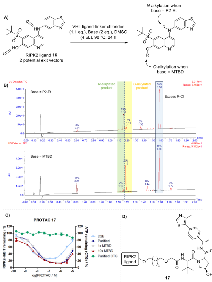
Scheme 5: A) Alkylation library carried out in D2B; B) Selective alkylation observed by LCMS when using P2-Et and MTBD as bases in 1536-well plate format; C) Curves from HiBIT and CTG assays for D2B samples (N=3), purified samples (N=2), and spiking experiments of purified PROTAC with MTBD (N=2); error bars represent SEM; D) Structure of RIPK2 PROTAC 17 .
