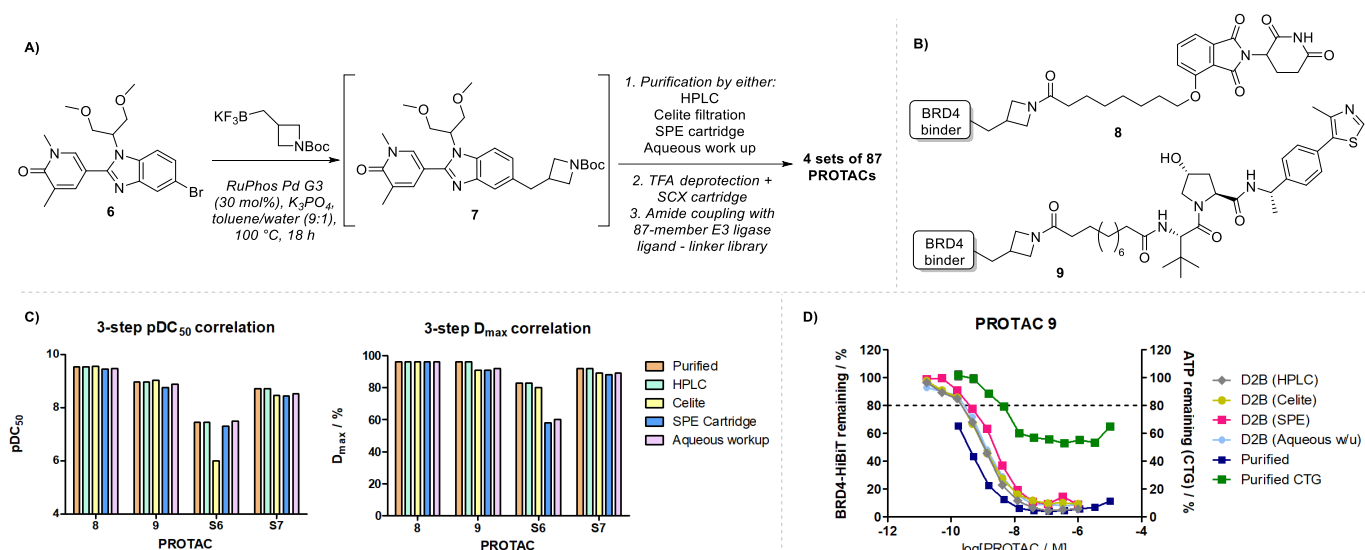
Scheme 3: A) Multistep process carried out in D2B; B) Exemplar resynthesised hits from library; C) Correlation between biological evaluation data obtained for different purification methods, where ‘purified’ data represents entirely purified samples, and other methods indicated correspond to purification method after the sp^2 - sp^3 cross-coupling reaction; D) Curves from HiBIT and CTG assays for D2B samples corresponding to each purification method (N=1) and purified samples (N=2). Error bars represent SEM.
