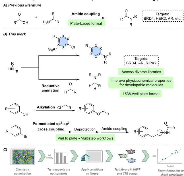
Figure 1 – A) Previous PROTAC direct-to-biology (D2B) work in the literature; B) This work describes the expansion of PROTAC D2B to additional chemical transformations with multiple protein-of-interest (POI) targets; C) Approach to identifying new reaction conditions for D2B.
