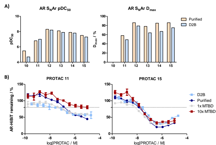
Figure 4 - A) Correlation between crude and purified samples; B) Curves from HiBiT assay for D2B samples, purified samples, and spiking experiments of purified PROTAC with MTBD – data is N=2 and error bars represent SEM.
