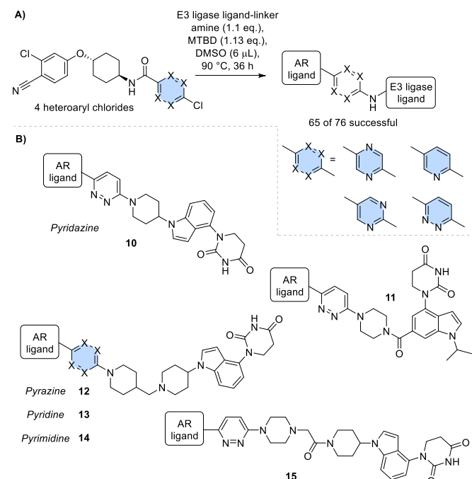
Scheme 4 - A) Nucleophilic aromatic substitution ( S_NAr ) library carried out in D2B; B) Exemplar resynthesised hits from library.
