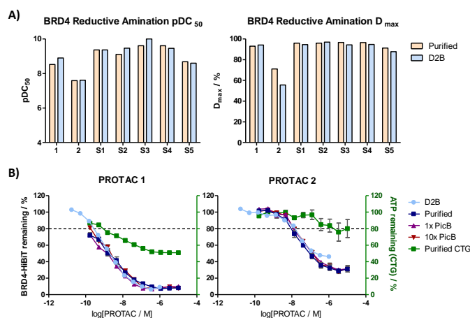
Figure 2 - A) Correlation between crude and purified samples; B) Curves from HiBiT and CTG assays for D2B samples (N=1), purified samples (N=2), and spiking experiments of purified PROTAC with picoline borane (PicB) (N=2). Error bars represent SEM.
