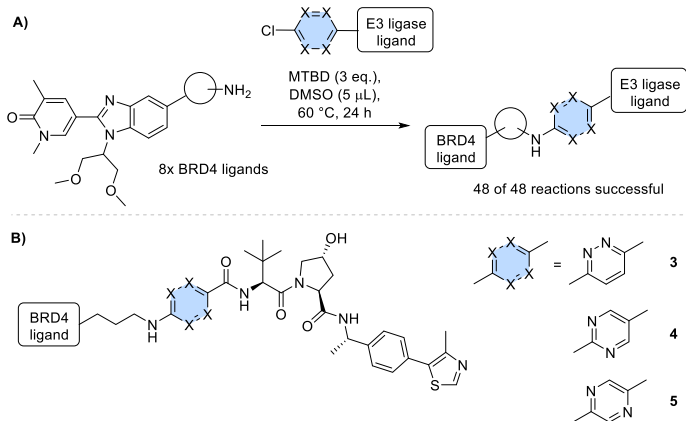
Scheme 2 - A) Nucleophilic aromatic substitution ( S_NAr ) library carried out in D2B; B) Exemplar resynthesised hits from library.
