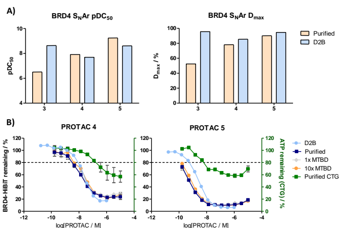
Figure 3 - A) Correlation between crude and purified samples; B) Curves from HiBiT and CTG assays for D2B samples (N=1), purified samples (N=2), and spiking experiments of purified PROTAC with MTBD (N=2). Error bars represent SEM.
