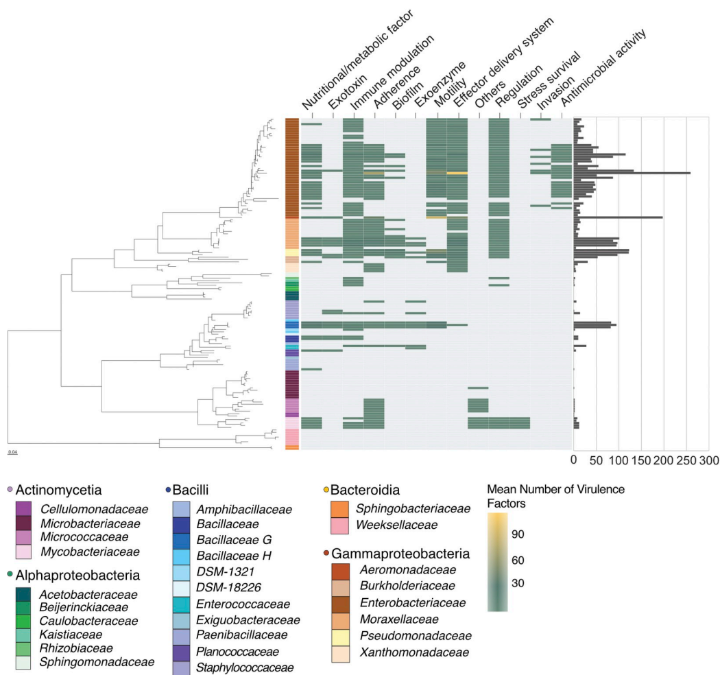
Fig 3. Heatmap of the distribution of virulence factors across all MosAIC genomes. Genes fall within one of 13 different categories (top). The guidance tree on the left is a maximum likelihood tree built using IQ-TREE2 and Baarnap-predicted 16S rRNA gene sequences from species clusters defined with dRep. Tiles denote the mean number of virulence factor genes identified within a given species cluster, following a gradient from blue (low) to yellow (high). Grey tiles denote species clusters for which zero predicted virulence factor genes were identified. Bacterial families are colour-coded in the figure legend. The bar chart on the right shows the total number of genes identified within each species cluster. All code and data to recreate this figure can be found at https://github.com/MosAIC-Collection/MosAIC_V1 in the folder “05_Virulence_Factor_Analysis.” MosAIC, Mosquito-Associated Isolate Collection.
