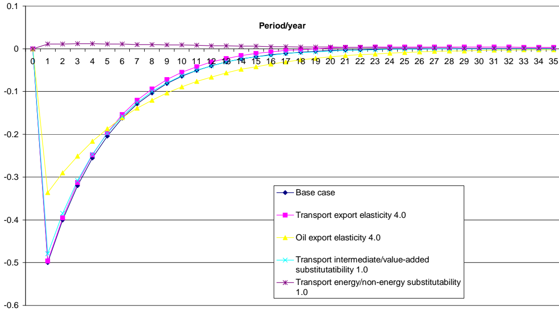
Figure 5. Sensitivity of Oil sector capital rental rate results to key parameter values (% change from base)
