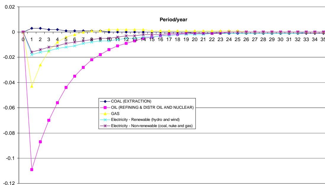
Figure 2. Impact of a 5% energy efficiency improvement in the Scottish Transport sector on output prices in Scottish energy supply sectors (% change from base)
