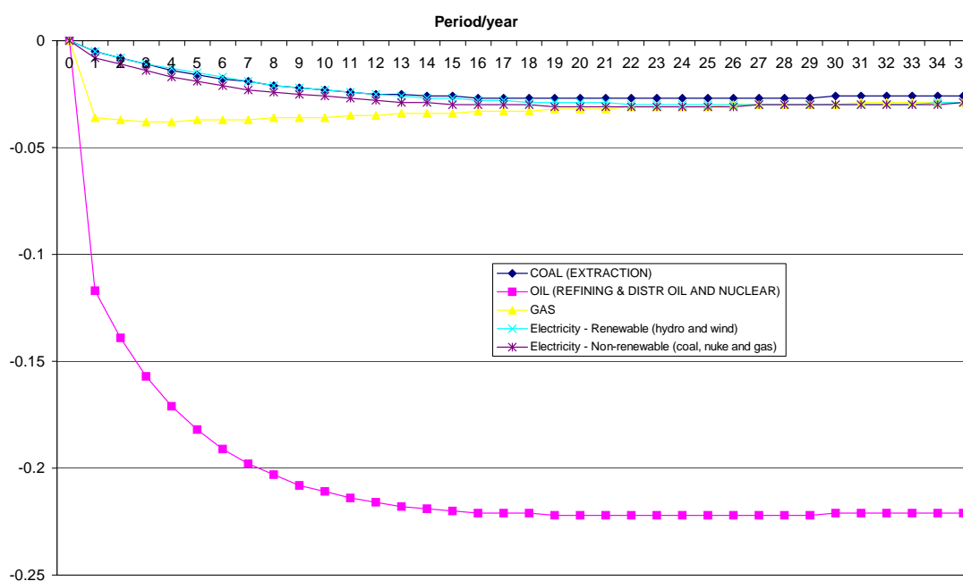
Figure 3. Impact of a 5% increase in energy efficiency in the Scottish Transport sector on output in the Scottish energy supply sectors (% change from base)
