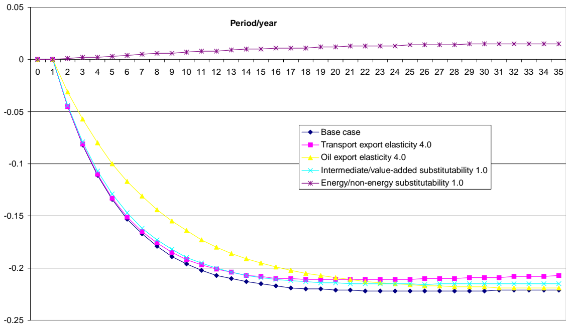
Figure 6. Sensitivity of Oil sector capital stock results to key parameter values
