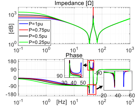
Fig.12 MMC3 DC impedances with different power flows.
