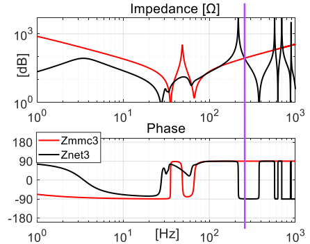
Fig. 18 The DC impedances with HTS cables at low transmitted power.
