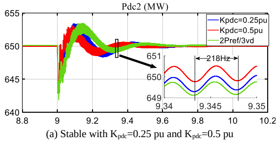
(a) Stable with K_{pdc}=0.25 pu and K_{pdc}=0.5 pu
