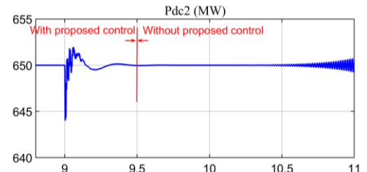
Fig. 22 With and without proposed control when K_{pdc}=1 .
