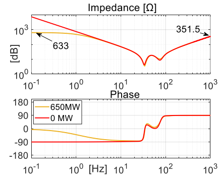
Fig. 17 MMC2 DC impedances with different transmitted power.
