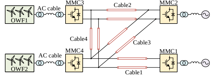
Fig. 1 Meshed four-terminal DC network
