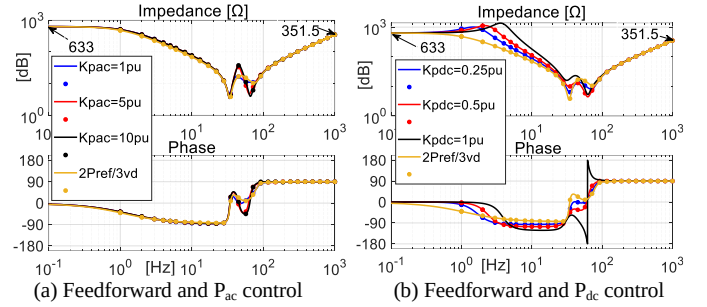
Fig. 8 MMC2 DC impedances with different control and parameters
