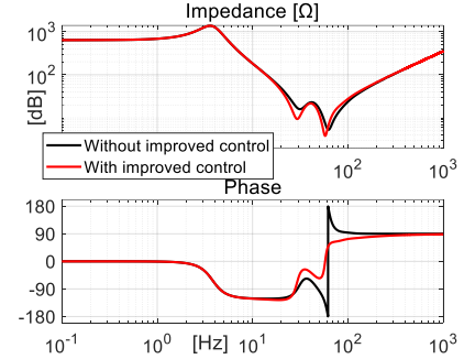
Fig. 21 Z_{\text{MMC2}} with and without proposed control.
