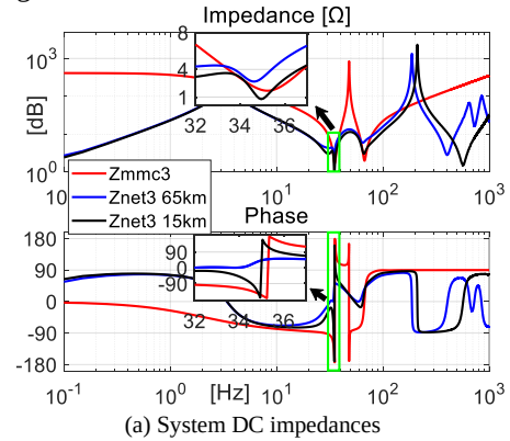
(a) System DC impedances
