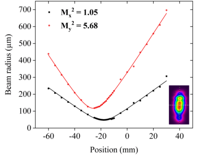
Fig. 3. Measurements of the output beam radius around the focus, for the x (black) and y (red) axes, before addition of the intracavity slits. Solid lines show the hyperbolic fit-function used to derive the annotated M^2 values. A profile of the collimated beam is included for reference.
