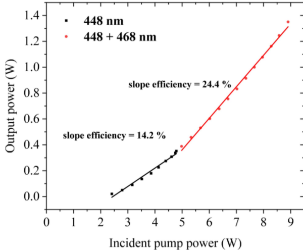
Fig. 2. Power transfer of the Ti:sapphire resonator before the addition of the intracavity slits.
