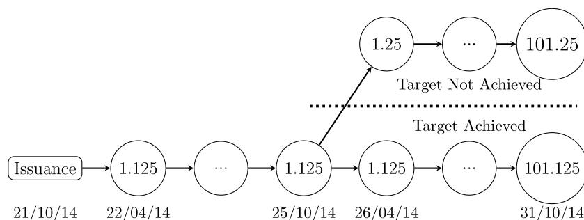
Fig. 1. SLB issued by General Mills in 2021. This figure illustrates the possible cash flows of the SLB issued by General Mills on October 14, 2021. The bond has a fixed semi-annual coupon of 1.125% and if General Mills fails to achieve a target reduction of 21% in scope 1 and scope 2 greenhouse gas emissions by 2025, the semi-annual coupon increases by 0.125%.
