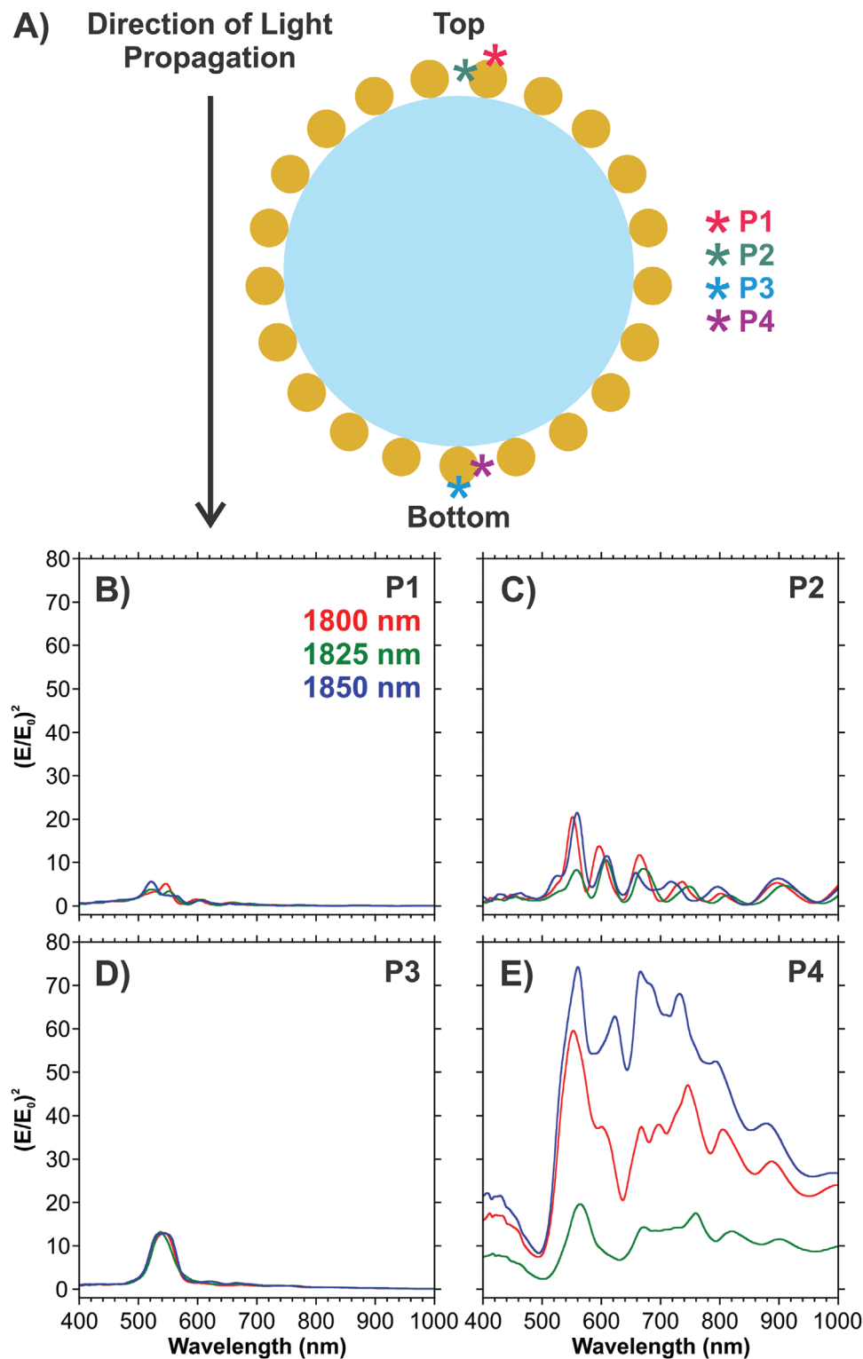
Figure 4. A) Representative schematic detailing where the electric field monitors are positioned with respect to a SiO 2 rod decorated with AuNPs and the direction of light propagation indicated. The top of the rod corresponds to the area nearest to the plane wave light source, and the bottom is the furthest away from it. B–D) FDTD calculated wavelength-dependent electromagnetic field intensities taken at the top and bottom of an 1800, 1825, and 1850 nm diameter SiO 2 rod decorated with AuNPs.
