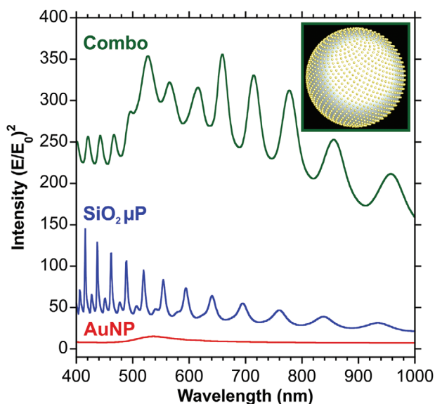
Figure 3. Finite-difference time-domain (FDTD) calculated wavelength-dependent electromagnetic field intensities for 50 nm AuNPs, a 2000 nm diameter SiO 2 microparticle (μP), and the SiO 2 μP decorated with the AuNPs arranged in a Fibonacci spiral configuration (Combo). The electric field intensities were determined by placing a monitor 1 nm away from the AuNP surface along the axis of the polarization, the base of the SiO 2 μP, and the bottom most AuNP, respectively.
