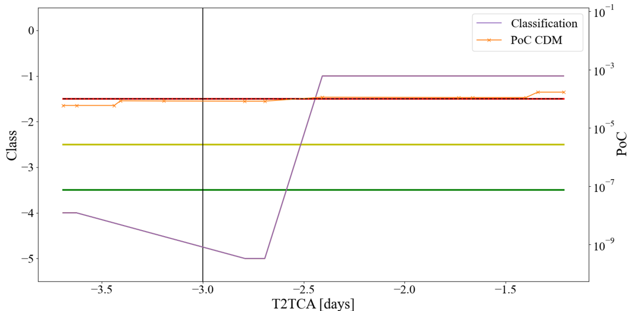
Fig. 10 Collision risk assessment for Event #1: High-risk event. Solid narrow lines: evidence-based classification with different number of \alpha -cuts: \#\alpha -cuts = \{1, 2, 3, 4, 5, 7\} (note that they overlap each other, so only \#\alpha -cuts = 7 is visible in solid purple). Crossed-solid line: PoC in the CDMs used by SDO for assessment. Horizontal thick lines: evidence approach safety bands: green, low risk-uncertain boundary; yellow, uncertain-high risk boundary; red, mid term high risk-long term high risk boundary. Dashed black line: Risk threshold (overlapping evidence-based high-risk boundary). Vertical black line: decision time threshold T_1 .
