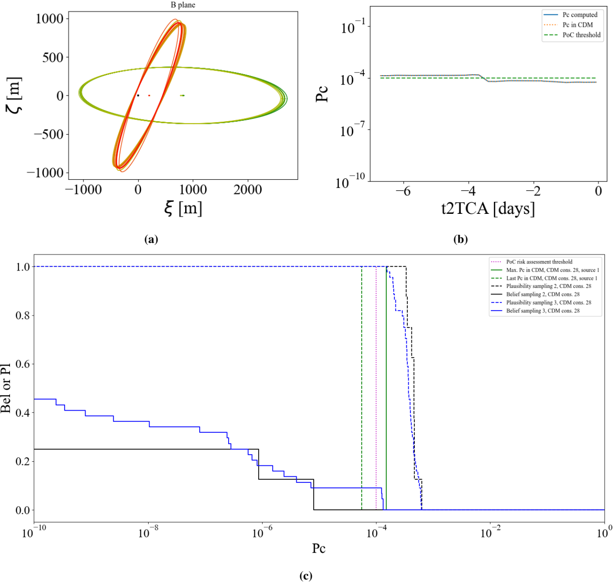
Fig. 23 Conjunction event with conflicting CDMs: a) evolution of the relative position distribution on the impact plane, b) evolution of the PoC, c) Pl and Bel curves of the whole CDMs sequence.
