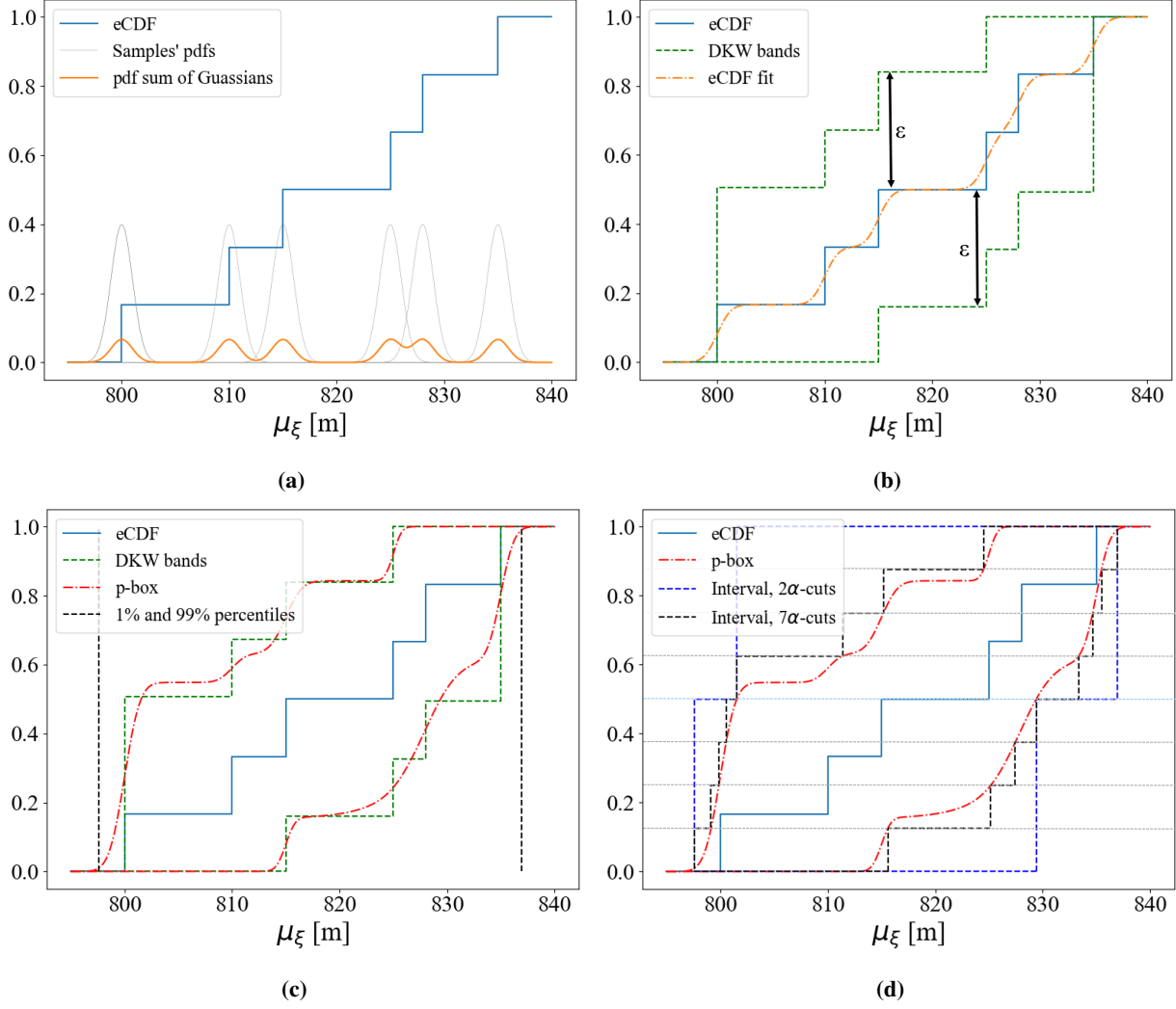
Fig. 2 Example of intervals derivation from the eCDF. (a) eCDF (solid blue), individual sample's Gaussian pdf distributions (solid grey), pdf of the sum of Gaussian distributions for the eCDF fit (solid orange) (b) eCDF (solid blue), DKW bands (dashed green), fitted eCDF with weighted sum of Gaussian distributions (dashed-pointed orange). (c) eCDF (solid blue), DKW bands (dashed green), p-box optimising the weighted sum of Gaussian distributions (dashed-pointed red), 1% and 99% percentiles (vertical dotted black lines). (d) eCDF (solid blue), p-box (dashed-pointed red), 1 \alpha -cut 2 intervals' PI and Bel (dashed blue), 7 \alpha -cuts 8 intervals' PI and Bel (dashed black). Dotted thin horizontal lines for the \alpha -cuts: light blue at 0.5 for the 2 intervals partition, grey lines spaced 0.125 for the 8 intervals partition.
