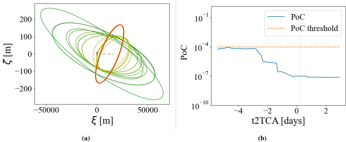
Fig. 15 CDM information for example in Event #3: Uncertain event. (a) Uncertain ellipses in the sequence of CDMs. Green ellipses correspond to earlier CDMs, and red ellipses to later CDMs. (b) Evolution of the PoC in the CDMs with the time to the TCA. Blue solid line: PoC; orange dashed line: PoC threshold, vertical dashed grey line: TCA.
