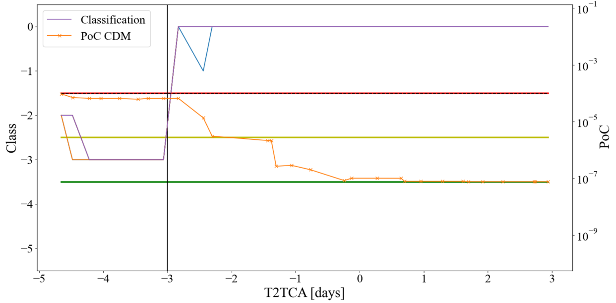
Fig. 18 Collision risk assessment for Event #3: Uncertain event. Solid narrow lines: evidence-based classification with different number of \alpha -cuts: \#\alpha\text{-cuts} = \{1, 2, 3, 4, 5, 7\} (note that they overlap each other, so only \#\alpha\text{-cuts} = 7 is visible for all t2TCA in solid purple; \#\alpha\text{-cuts} = 1 in solid blue and \#\alpha\text{-cuts} = 2 in solid orange are visible at one t2TCA each). Crossed-solid line: PoC in the CDMs used by SDO for assessment. Horizontal thick lines: evidence approach safety bands: green, low risk-uncertain boundary; yellow, uncertain-high risk boundary; red, mid term high risk-long term high risk boundary. Dashed black line: Risk threshold (overlapping evidence-based high-risk boundary). Vertical black line: decision time threshold T_1 . Vertical dashed grey line: TCA.
