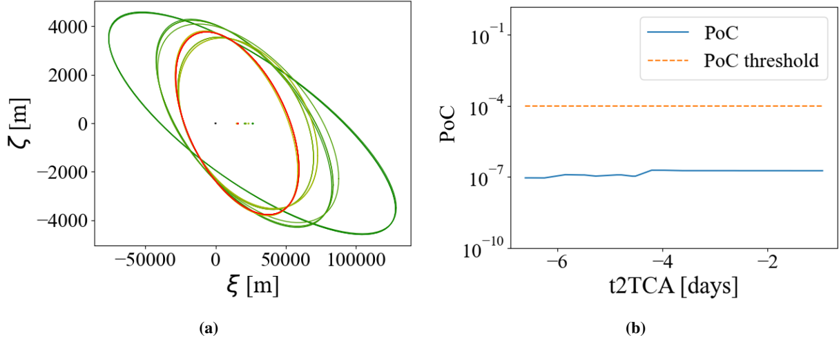
Fig. 11 CDM information for example in Event #2: Low-risk event. (a) Uncertain ellipses in the sequence of CDMs. Green ellipses correspond to earlier CDMs, and red ellipses to later CDMs. (b) Evolution of the PoC in the CDMs with the time to the TCA. Blue solid line: PoC; orange dashed line: PoC threshold.
