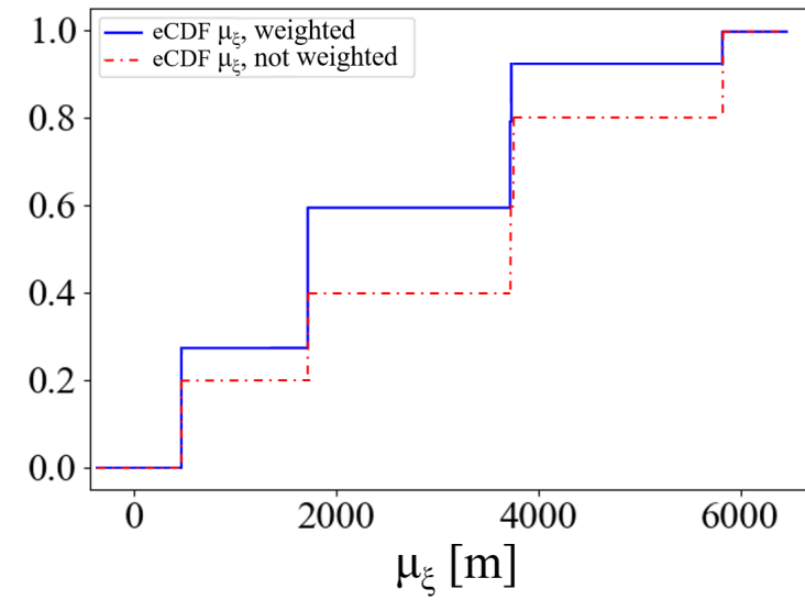
Fig. 4 eCDF for \mu_\xi weighing the samples (blue) and with samples equally weighted (dashed red).
