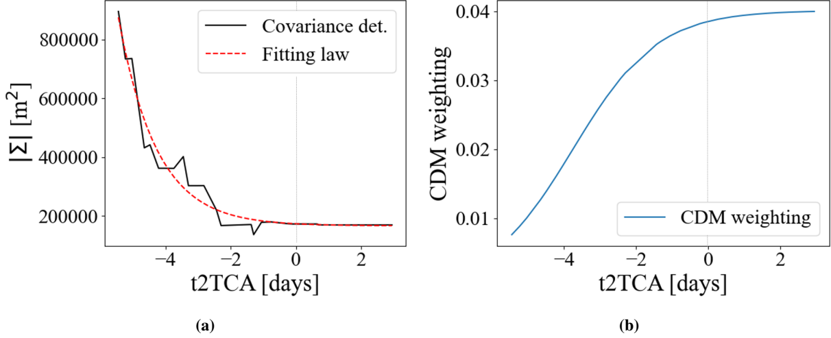
Fig. 16 Fitting law to weight the CDMs after having received the whole sequence in Event #3: Uncertain event. (a) Solid black line: value of the determinant from the CDMs, dashed red line: fitting law of the covariance matrix determinant. Vertical dashed grey line: TCA. (b) Weight of the CDMs as a function of the time to the TCA. Vertical dashed grey line: TCA.
