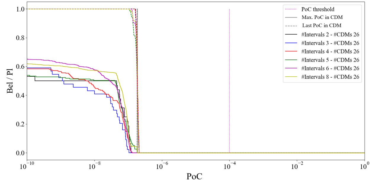
Fig. 13 Pl and Bel of the PoC after having received the whole sequence of CDMs Event #2: Low-risk event. Solid vertical grey line: maximum PoC in the sequence, dashed vertical grey line: PoC of last CDM, pointed purple line: PoC threshold. For the rest of the colours: Belief in solid lines and Plausibility in dashed lines. Black: 1 \alpha -cut per variable (2 intervals per variable, 32 FEs), blue: 2 \alpha -cuts, red: 3 \alpha -cuts, green: 4 \alpha -cuts, purple: 5 \alpha -cuts, yellow: 7 \alpha -cuts.
