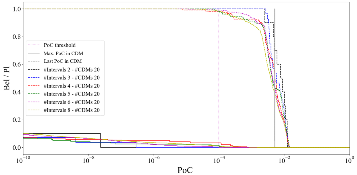
Fig. 21 Pl and Bel of the PoC after having received the whole sequence of CDMs Event #4. Solid vertical grey line: maximum PoC in the sequence, dashed vertical grey line: PoC of last CDM, pointed purple line: PoC threshold. For the rest of the colours: Belief in solid lines and Plausibility in dashed lines. Black: 1 \alpha -cut per variable (2 intervals per variable, 32 FEs), blue: 2 \alpha -cuts, red: 3 \alpha -cuts, green: 4 \alpha -cuts, purple: 5 \alpha -cuts, yellow: 7 \alpha -cuts.
