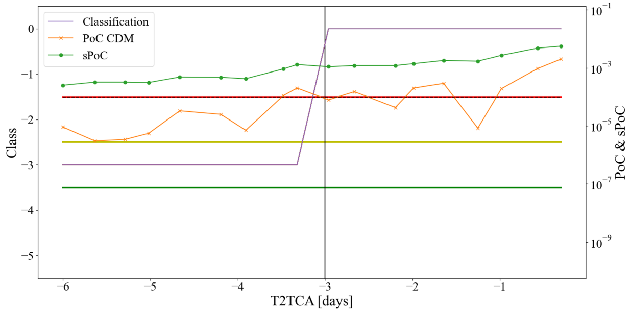
Fig. 22 Collision risk assessment for Event #4. Solid narrow lines: evidence-based classification with different number of \alpha -cuts: \#\alpha -cuts = \{1, 2, 3, 4, 5, 7\} (note that they overlap each other, so only \#\alpha -cuts = 7 is visible in solid purple). Crossed-solid line: PoC in the CDMs used by SDO for assessment. Horizontal thick lines: evidence approach safety bands: green, low risk-uncertain boundary; yellow, uncertain-high risk boundary; red, mid-term high risk-long term high risk boundary. Dashed black line: Risk threshold (overlapping evidence-based high-risk boundary). Vertical black line: decision time threshold T_1 .
