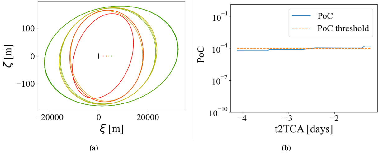
Fig. 7 CDM information for example in Event #1: High-risk event. (a) Uncertain ellipses in the sequence of CDMs. Green ellipses correspond to earlier CDMs, and red ellipses to later CDMs. (b) Evolution of the PoC in the CDMs with the time to the TCA. Blue solid line: PoC; orange dashed line: PoC threshold.
