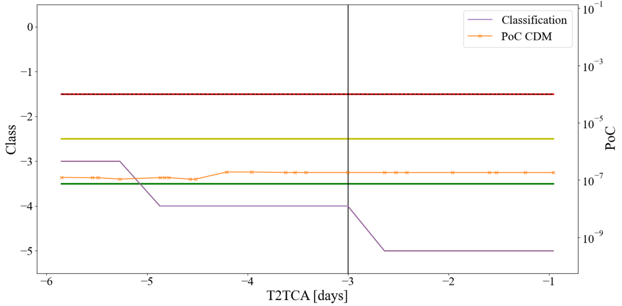
Fig. 14 Collision risk assessment for Event #2: Low-risk event. Solid narrow lines: evidence-based classification with different number of \alpha -cuts: \#\alpha\text{-cuts} = \{1, 2, 3, 4, 5, 7\} (note that they overlap each other, so only \#\alpha\text{-cuts} = 7 is visible in solid purple). Crossed-solid line: PoC in the CDMs used by SDO for assessment. Horizontal thick lines: evidence approach safety bands: green, low risk-uncertain boundary; yellow, uncertain-high risk boundary; red, mid term high risk-long term high risk boundary. Dashed black line: Risk threshold (overlapping evidence-based high-risk boundary). Vertical black line: decision time threshold.
