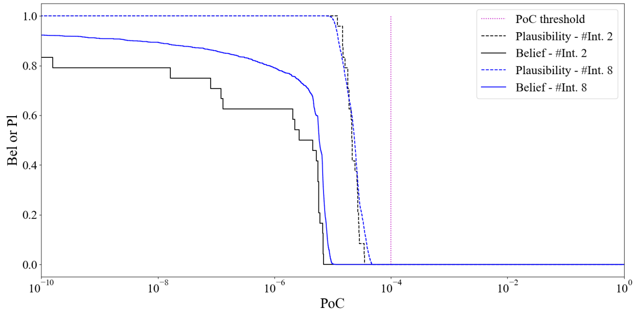
Fig. 5 Plausibility and Belief of PoC \geq PoC_0 . Black: 1 \alpha -cut (two intervals) per variable, 32 FEs. Blue: 7 \alpha -cut (eight intervals) per variable, 32768 FEs. Solid lines: belief. Dashed lines: plausibility. Dotted purple vertical line: PoC_0 .
