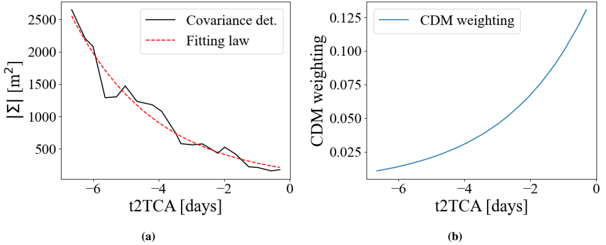
Fig. 20 Fitting law to weight the CDMs after having received the whole sequence in Event #4. (a) Solid black line: value of the determinant from the CDMs, dashed red line: fitting law of the covariance matrix determinant. (b) Weight of the CDMs as a function of the time to the TCA.
