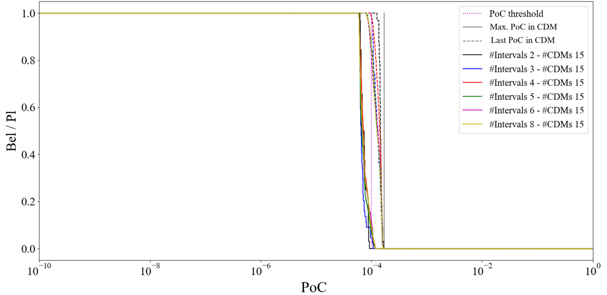
Fig. 9 Pl and Bel of the PoC after having received the whole sequence of CDMs Event #1: High-risk event. Solid vertical grey line: maximum PoC in the sequence, dashed vertical grey line: PoC of last CDM, pointed purple line: PoC threshold. For the rest of the colours: Belief in solid lines and Plausibility in dashed lines. Black: 1 \alpha -cut per variable (2 intervals per variable, 32 FEs), blue: 2 \alpha -cuts, red: 3 \alpha -cuts, green: 4 \alpha -cuts, purple: 5 \alpha -cuts, yellow: 7 \alpha -cuts.
