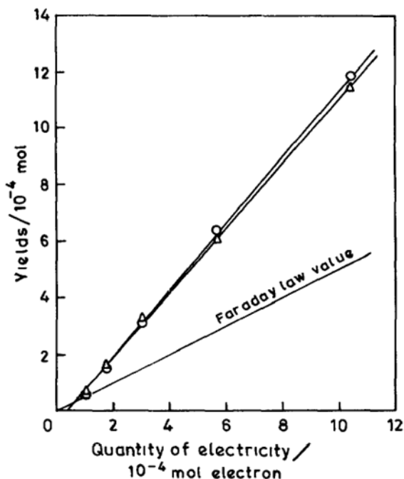
Figure 11: Variation of the yields of \text{H}_2 (o), and combined \text{H}_2\text{O}_2 (triangle) and \text{O}_2(^1\Delta) as a function of the charged transferred to the liquid during contact glow discharge electrolysis. Reproduced with permission from [238].
