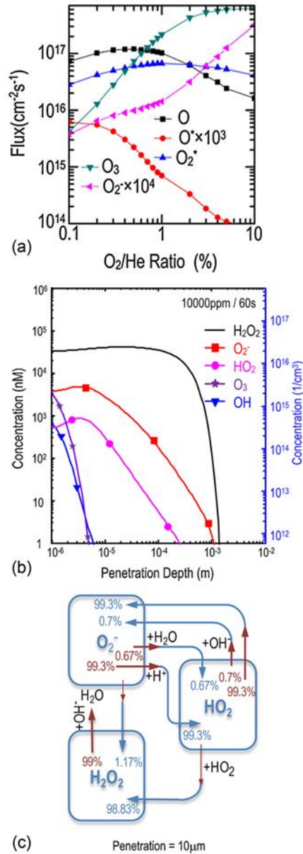
Figure 27: Gas and liquid phase reactant densities from an atmospheric pressure plasma sustained in \text{He}/\text{O}_2 in contact with water. (a) Fluxes of ROS to the surface of the water for gas phase \text{O}_2 concentrations of 0–10 %. (b) In liquid densities of ROS as a function of distance of penetration into the bulk liquid bulk for \text{He}/\text{O}_2 = 99/1 . (c) The pathway chain map for key ROS is shown for 10 mm into the liquid. The percentage for each pathway indicates the contribution for generation or loss of the species. Reproduced with permission from [188].
