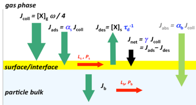
Figure 9: Schematic of key processes and fluxes in the gas uptake by atmospheric particles: gas kinetic flux of surface collisions ( J_{\text{coll}} ), adsorption onto the particle surface ( J_{\text{ads}} ), absorption into the particle bulk ( J_{\text{abs}} ), desorption from the surface ( J_{\text{des}} ), and net uptake by the condensed phase ( J_{\text{net}} ). The red arrows indicate production and loss of chemical species by reactions at the particle surface ( P_s , L_s ) or in the particle bulk ( P_b , L_b ). [X]_g and [X]_s are the gas and surface concentrations. Reproduced with permission from [156].
