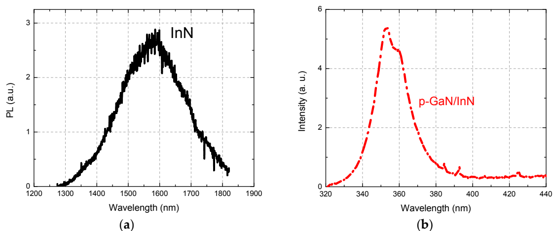
Figure 4. Room-temperature photoluminescence (PL) spectra of InN/p-GaN heterojunction grown on sapphire substrates: (a) near-infrared from 1200 nm to 1900 nm, (b) UV range from 320 nm to 440 nm.
