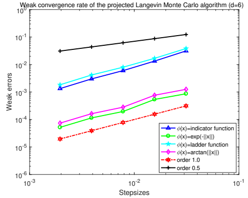
Figure 2: Weak convergence rates of PLMC algorithm for the double well model ( d = 6 )
