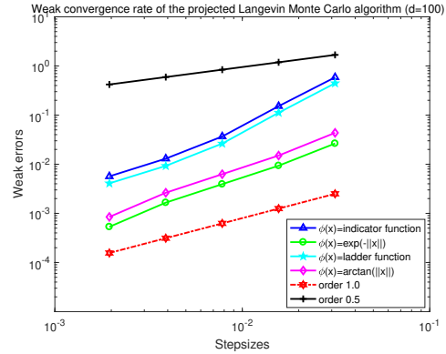
Figure 5: Weak convergence rates of PLMC algorithm for the double well model ( d = 100 )
