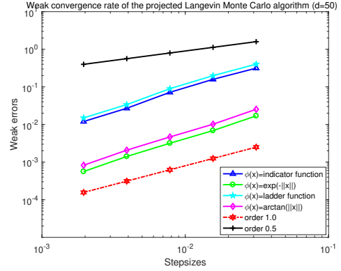
Figure 4: Weak convergence rates of PLMC algorithm for the double well model ( d = 50 )
