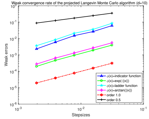
Figure 3: Weak convergence rates of PLMC algorithm for the double well model ( d = 10 )
