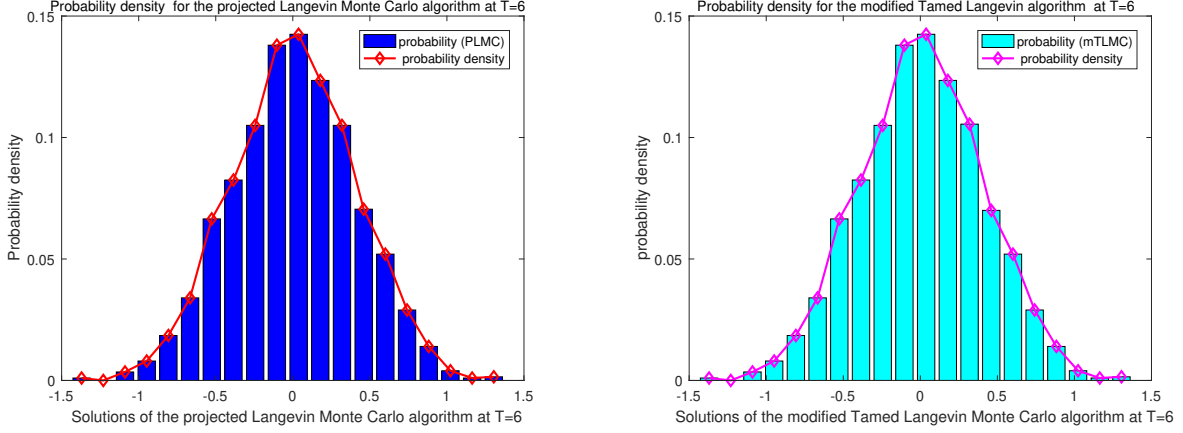
Figure 1: Probability density of the first component of the double-well model.
