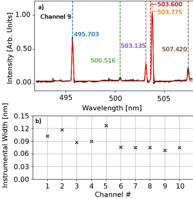
Figure 3. (a) Recorded (black) and fitted (red) spectra from a neon calibration lamp for one representative spectrometer channel. (b) The width of the fitted Gaussian instrument function for each spectrometer channel.
