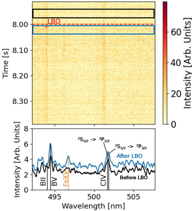
Figure 8. Recorded spectrum following Fe LBO injection into a plasma with no neutral beam injection. The top plot shows the signal intensity in the color scale. Passive emission prior-to (after) the Fe injection is time-averaged over the range specified by the black (blue) box and plotted in the bottom window. (Program #20230314.41).
