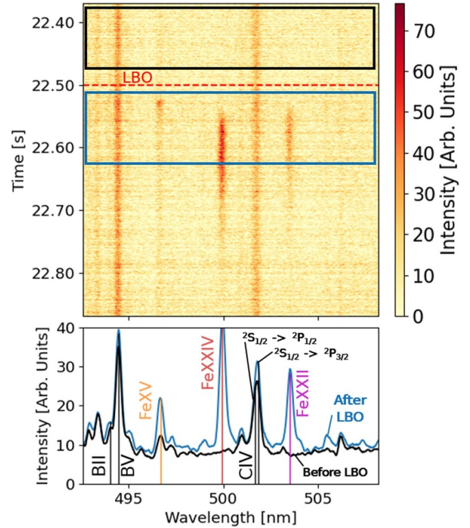
Figure 5. Spectrum following laser blow-off (LBO) injection of Fe into plasma with continuous NBI (Program # 20230314.26). The top plot shows signal intensity vs time and wavelength. Impurity emission prior-to (after) the LBO injection is time-averaged over the range specified by the black (blue) box and shown in the bottom window. The Fe XV overlaps with an Ar XV line explaining the emission before the LBO.
