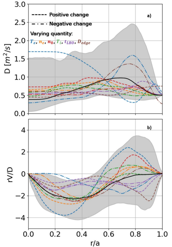
Figure 14. Median (a) diffusion and (b) peaking ratio profiles for varied inputs to the Bayesian inference model with color coding depicting which parameter is varied. Positive changes to the parameter of interest are given in dashed lines while negative changes are given in dot-dashed lines. The base case considered in the previous section is shown in solid black with fitting uncertainty shown in shaded grey.
