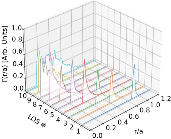
Figure 2. Radial resolution functions calculated from pyFIDASIM. Each function is normalized such that it integrates to 1. Note that lines of sight 8–10 exhibit lesser spatial localization as they are more oblique to the beam axis.
