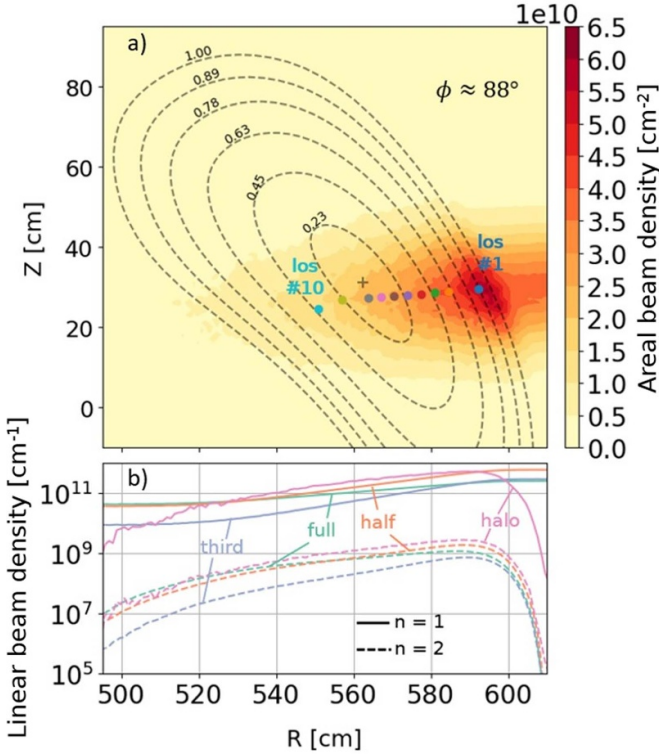
Figure 1. (a) Approximate locations of intersection between ten of the new CXRS diagnostic lines of sight and the 50 keV neutral beam. Shown in color-scale is the beam density integrated over the toroidal direction. (b) Attenuation of the various beam components for energy levels n = 1 and n = 2 . Plotted densities are integrated over both the toroidal and Z directions.
