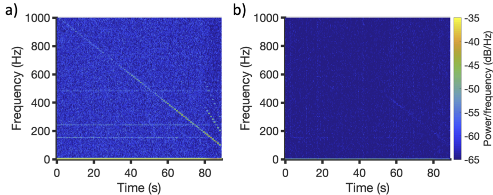
Fig. 4. Spectrogram plots of sound recovery from our laser microphone setup. A linear chirp ranging from 1000 to 100 Hz is played through the loudspeaker and the Fourier transform of the intensity signal from the PMT is plotted for (a) 30 beams with optimised position and phase and (b) the same 30 beams with optimised position and randomised phase.
