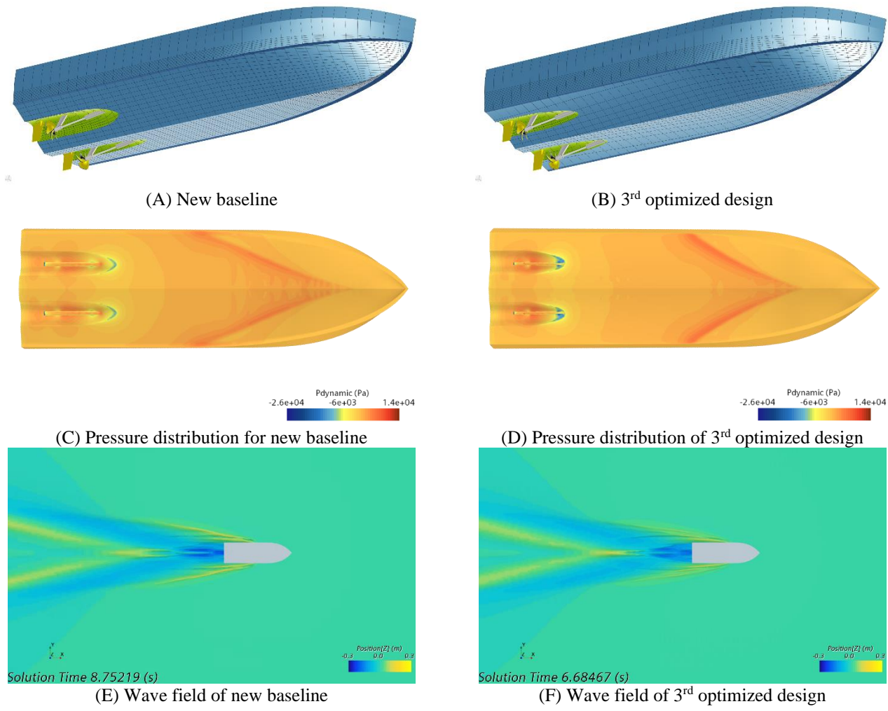
Figure 14: Parametric model built from assembly of bare hull, tunnel and propulsion train and associated flow fields
