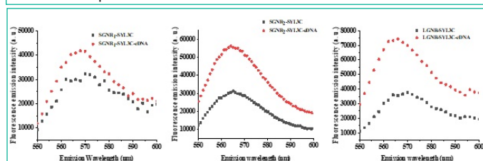
Figure 2: The fluorescence emission spectra of Cy3 in the gold nanorods nanoprobe before and after hybridization; (a) SGNR 1 -SYL3C nanoprobe, (b) SGNR 2 -SYL3C nanoprobe (c) LGNR-SYL3C nanoprobe.
