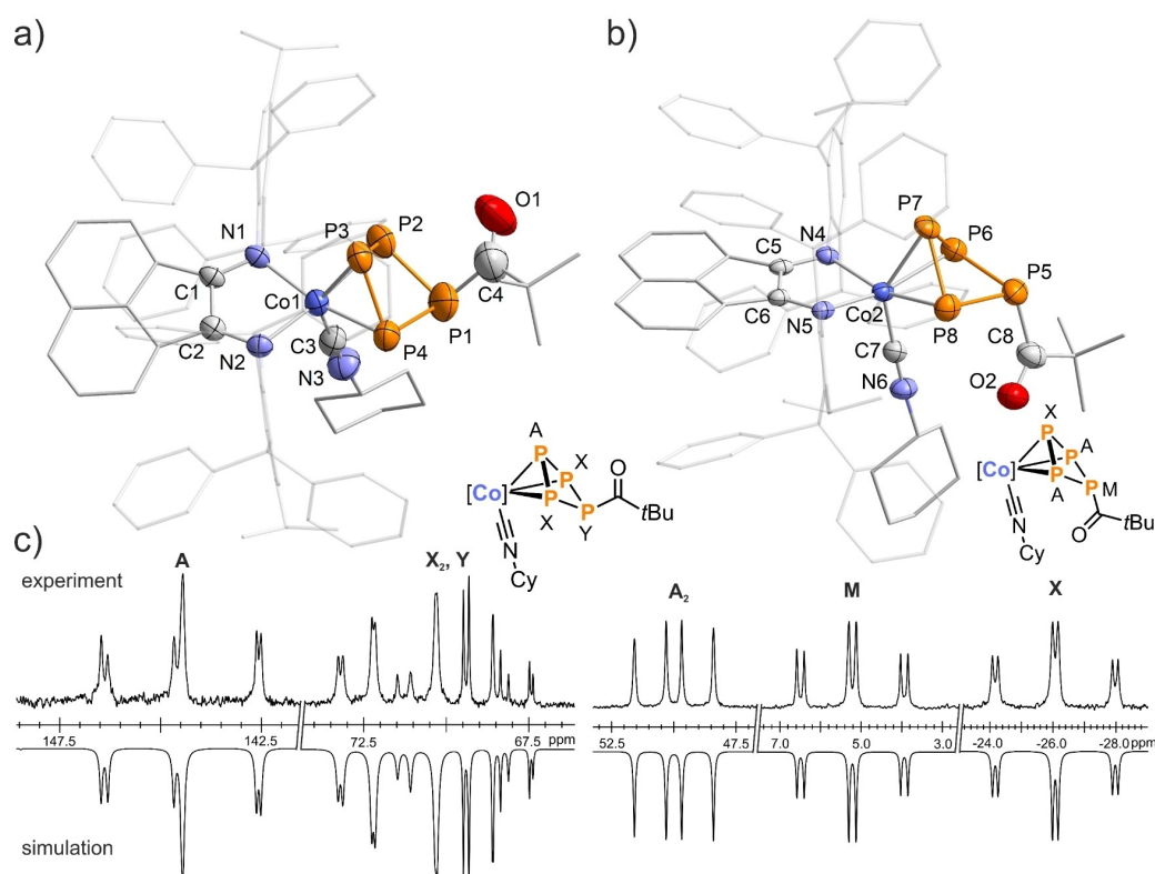
Figure 4. Solid-state molecular structures of a) endo -[( \text{Ar}^*\text{BIAN})\text{Co}(\text{CyNC})(\eta^3\text{-P}_4\text{C}(\text{O})t\text{Bu})] ( endo - 6a ) and b) exo -[( \text{Ar}^*\text{BIAN})\text{Co}(\text{CyNC})(\eta^3\text{-P}_4\text{C}(\text{O})t\text{Bu})] ( exo - 6a ) in the co-crystal; [45] thermal ellipsoids are shown at the 50% probability level; hydrogen atoms, disorder and non-coordinating solvent molecules are omitted for clarity. Selected bond lengths [Å] and angles [°] of endo - 6a : P1–P2 2.218(3), P1–P4 2.232(3), P2–P3 2.191(2), P3–P4 2.165(3), Co1–P2 2.3000(2), Co1–P3 2.2983(2), Co1–P4 2.3027(2), Co1–C3–N3 178.4(5); c) experimental (upward) and simulated (downward) ^{31}\text{P}\{^1\text{H}\} NMR spectra of endo - 6a with nuclei assigned to an \text{AX}_2\text{Y} spin system: \delta(\text{P}_\text{A})=144.5 ppm, \delta(\text{P}_\text{X})=71.7 ppm, \delta(\text{P}_\text{Y})=68.6 ppm, ^1J_{\text{AX}}=-318 Hz, ^1J_{\text{XY}}=-165 Hz, ^2J_{\text{AY}}=-5 Hz; exo - 6a : \delta(\text{P}_\text{A})=50.0 ppm, \delta(\text{P}_\text{M})=5.2 ppm, \delta(\text{P}_\text{V})=-26.1 ppm, ^1J_{\text{AX}}=-308 Hz, ^1J_{\text{AM}}=-207 Hz, ^2J_{\text{MX}}=29 Hz.
