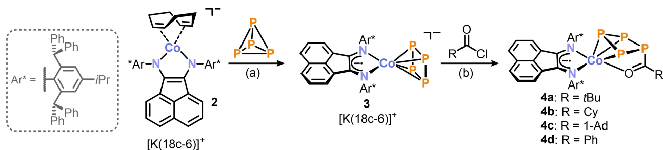
Scheme 1. Activation of \text{P}_4 by [\text{K}(\text{18c-6})]_2 and subsequent functionalization of the cyclo- \text{P}_4 unit in [\text{K}(\text{18c-6})]_3 with acyl chlorides (18c-6 = [18]-crown-6, \text{Ar}^* = 2,6 -dibenzhydryl-4-isopropylphenyl); reagents/by-products and conditions: a) +\text{P}_4/-1,5 cyclooctadiene (1,5-cod); THF, r.t., 1 d; b) +\text{RC}(\text{O})\text{Cl}/-[\text{K}(\text{18c-6})]\text{Cl} ; toluene, r.t., 1 d; yields: [\text{K}(\text{18c-6})]_2 : 77%, [\text{K}(\text{18c-6})]_3 : 63%, 4a : 58%, 4b : 54%, 4c : 66%, 4d : 67%.
