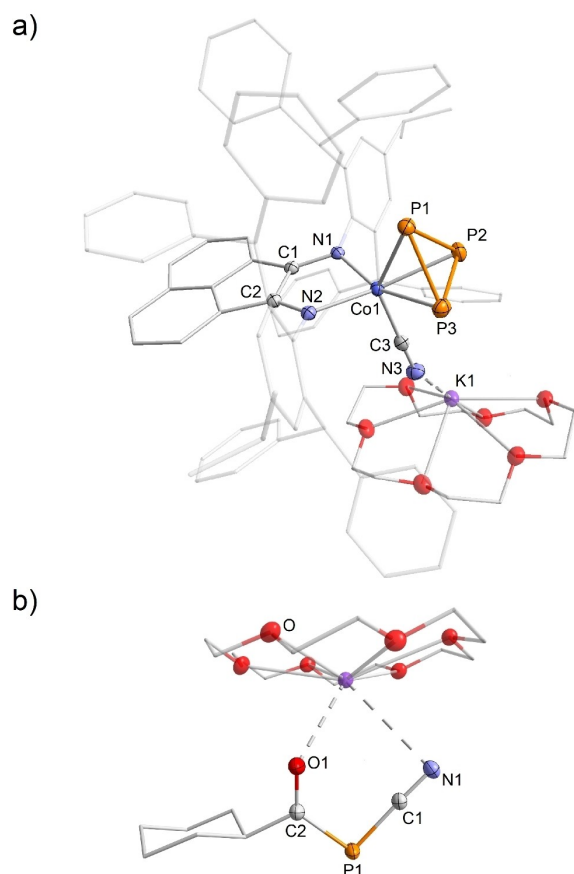
Figure 5. Solid-state molecular structures of a) [K(18c-6)][(Ar^*BIAN)Co(CN)(\eta^3-P_3)] ( [K(18c-6)]\mathbf{8} ) and b) K(18c-6)[CycC(O)PCN] ( [K(18c-6)]\mathbf{9b} ); [45] thermal ellipsoids are shown at the 50% probability level; hydrogen atoms and disorder are omitted for clarity. Selected bond lengths [Å] and angles [°] of [K(18c-6)]\mathbf{8} : P1–P2 2.1318(5), P1–P3 2.1306(5), P2–P3 2.1682(4), Co1–P1 2.3070(4), Co1–P2 2.3001(4), Co1–P3 2.3014(3), Co1–C3 1.9323(1), C1–N1 1.3211(2), C3–N3 1.1583(2), C1–C2 1.4486(2), K1–N3 2.9111(1), P1–P2–P3 59.396(2), P1–P3–P2 59.452(2), P2–P1–P3 61.152(2), Co1–C3–N3 177.83(1); [K(18c-6)]\mathbf{9b} : P1–C1 1.7789(1), P1–C2 1.7960(1), C1–N1 1.1519(2), C2–O1 1.2397(1), P1–C1–N1 176.77(9), C1–P1–C2 95.08(5).
