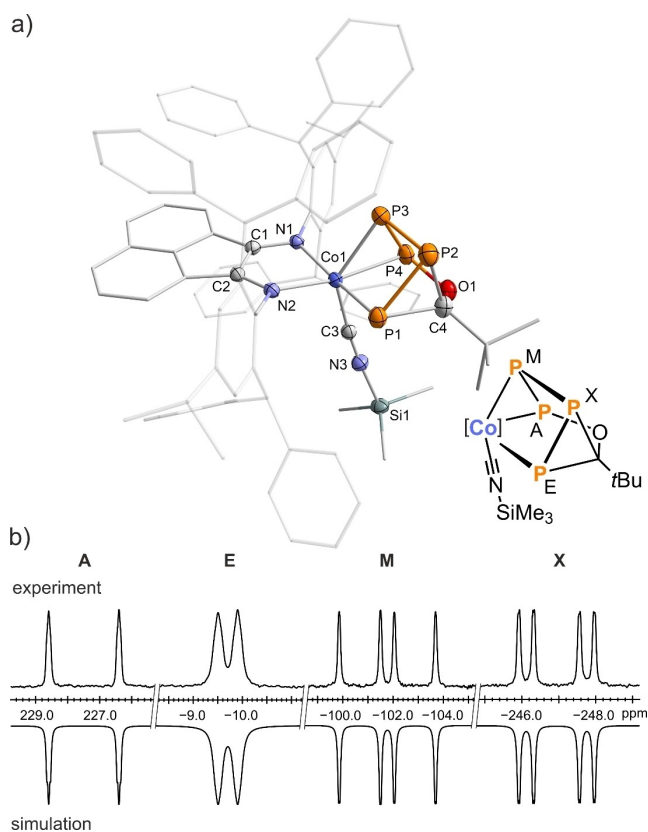
Figure 3. a) Solid-state molecular structure of [(Ar*BIAN)Co-(Me 3 SiNC)] ( 5a ); [45] thermal ellipsoids are shown at the 50% probability level; hydrogen atoms and disorder are omitted for clarity. Selected bond lengths [Å] and angles [°]: P1–P2 2.1961(1), P2–P3 2.207(1), P3–P4 2.1355(1), Co1–P1 2.2895(7), Co1–P3 2.3330(8), Co1–P4 2.2987(8), C4–O1 1.432(3), P4–O1 1.6722(2), Co1–C3 1.851(2), Co1–C3–N3 174.3(2), C3–N3–Si1 176.14(2); b) experimental (upward) and simulated (downward) 31 P{ 1 H} NMR spectra of 5a with nuclei assigned to an AEMX spin system: \delta(P_A) = 228.1 ppm, \delta(P_E) = -10.7 ppm, \delta(P_M) = -102.4 ppm, \delta(P_X) = -245.1 ppm, ^1J_{AM} = -355 Hz, ^1J_{MX} = -267 Hz, ^1J_{EX} = -64 Hz, ^2J_{AX} = 8 Hz, ^2J_{ME} = 9 Hz, ^3J_{AE} = -11 Hz. The spectra of the related compounds 5b–r are very similar (see SI, Figures S47–S52); [Co] = (Ar*BIAN)Co.
