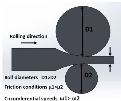
Fig. 16 Schematic of asymmetric rolling
