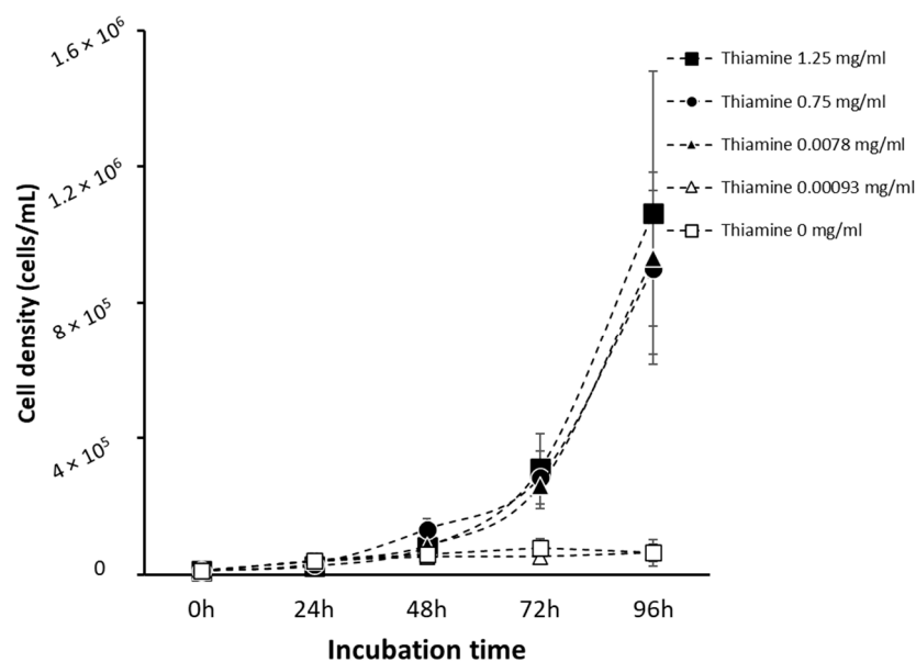
Figure 2. Growth curve of A. castellanii ( 1 \times 10^4 cells/mL) in chemically defined medium M20 containing variable levels of thiamine. Thiamine concentrations ranged from 1.25 mg/mL to 0 mg/mL. Cell density was estimated over 96 h in cells incubated with 1.25 mg/mL (closed square), 0.75 mg/mL (closed circle), 0.0078 mg/mL (closed triangle), 0.00093 mg/mL (open triangle), and 0 mg/mL (open square) of thiamine. Data are mean cell count \pm SD; n = 3 independent experiments performed in triplicates.
