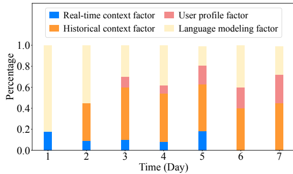
Fig. 15. The daily percentages of the four factors in phase 2.
