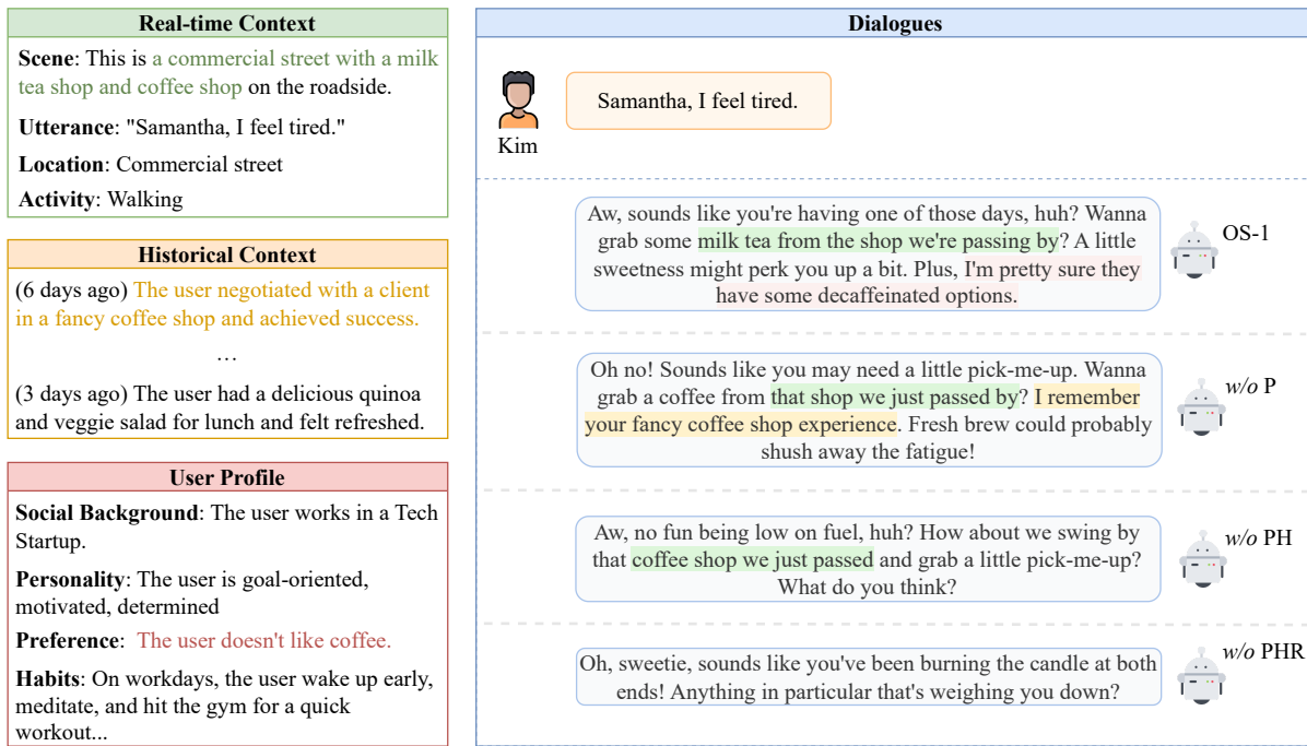
Fig. 9. A case of shop recommendation. Left: personal context captured by OS-1. Right: four dialogue sessions between a simulated user and four systems.
