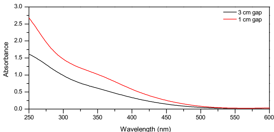
Fig. 4. The ultraviolet–visible spectra of copper oxide dispersions formed in ethanol when the gap between the electrodes is reduced from 3 cm (black line) to 1 cm (red line). (For interpretation of the references to colour in this figure legend, the reader is referred to the web version of this article.)
