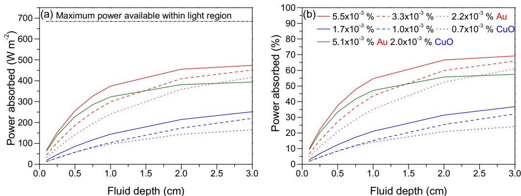
Fig. 8. The calculated power absorbed by nanofluids is determined for lengths scales ranging from 0.1 cm to 3 cm. (a) Power absorbed per m 2 is plotted from the solar irradiance spectra between 300 and 900 nm. (b) The percentage of power absorbed per m 2 was determined and charted.
