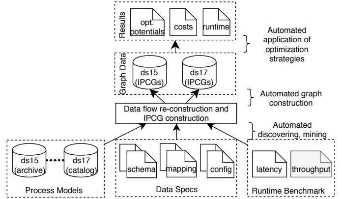
Figure 30: Pattern composition evaluation pipeline.
