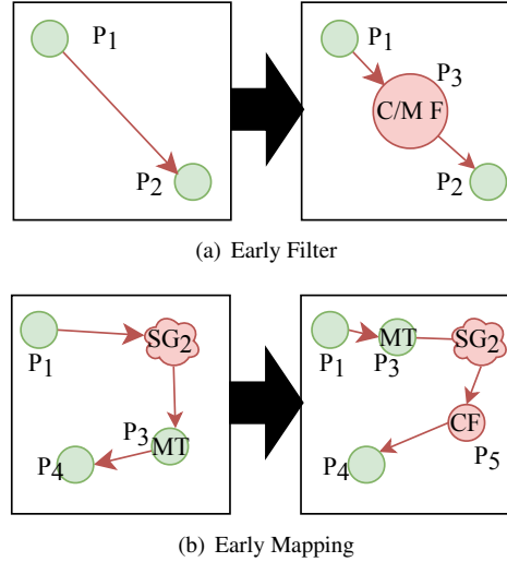
Figure 22: Rules for early-filter and early-mapping.
