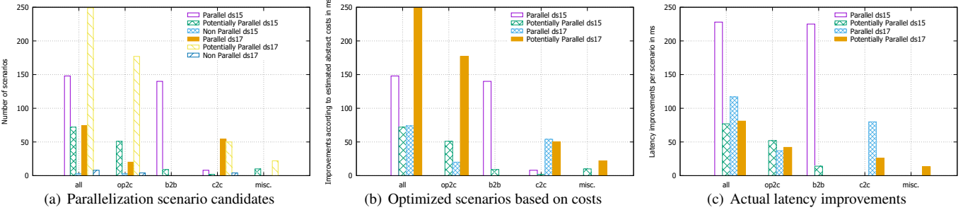
Figure 33: OS-3 “Sequence to parallel” optimization candidates on (a) integration flows, (b) optimization selection based on abstract cost model, and (3) actual latency improvements.
