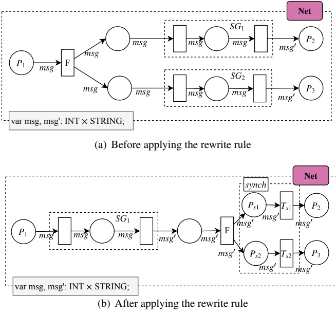
Figure 29: Timed db-net translation of IPCGs before and after applying the “combine sibling patterns” rewrite rule
