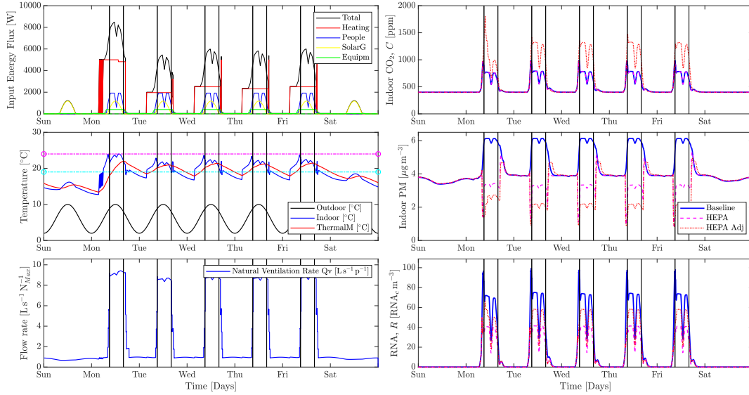
Figure 3: Simulation of winter-like conditions.
