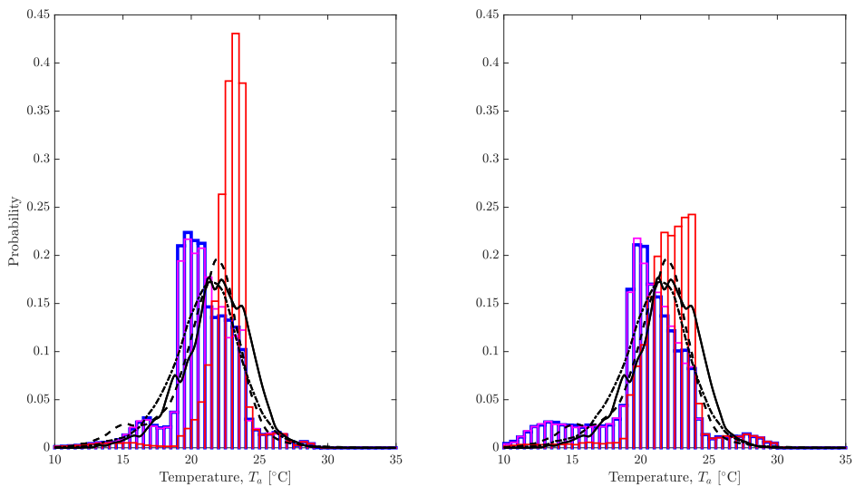
Figure 2: Histograms of the temperatures within the simulated classroom using the weather and \text{PM}_{2.5} data for Leeds: the left-hand pane shows the histograms of the modelled data from the Modern construction classroom and the right-hand pane those from the Victorian ear classroom; both panes include black curves illustrating the PDFs from the measured data (the solid curve marks data reported within Burrige et al. [29], the dashed curve that reported by Vouriot et al. [30], and the dashed-dotted line marks data from the SAMHE Project [65]). blue histograms illustrate the baseline cases, the magenta histograms mark the HEPA cases, and red the HEPA Adjusted cases.
