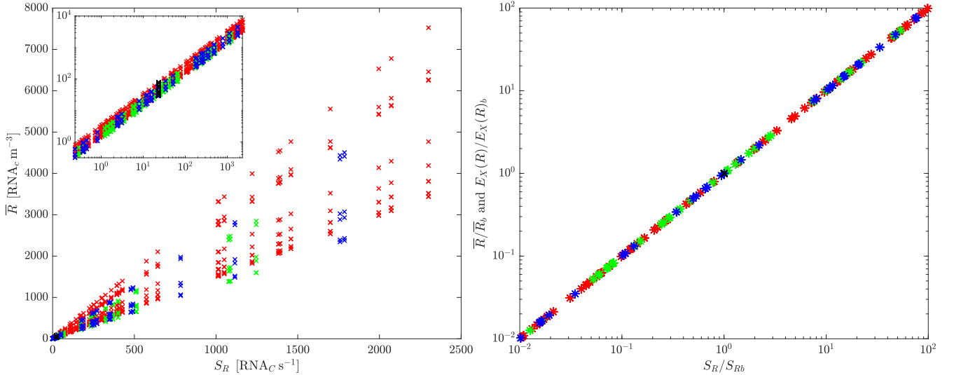
Figure 6: The variation in average concentration of RNA copies, and potential exposures, with the RNA source term, S_R = I p C_R . In each figure black crosses, \times , mark the results from the set of our 24 reported simulations and scenarios (i.e. for three HEPA based scenarios in both a Modern Construction and Victorian era classrooms, each simulated with year-long simulations using data for London and for Leeds, and Specified winter and summer conditions); all other data plotted, mark results from the 24 simulations and scenarios with differing values taken for the RNA source term. The RNA source term was randomly varied over four decades of magnitude and the red data marks 80 different RNA source term values each ran for the Specified winter and summer conditions, green data denotes results for the 40 values ran with year-long simulations using data for London, and blue data the 30 values using data for Leeds. The left-hand pane shows the data unscaled, within the same data is inset plotted on log-log axes. The right-hand pane shows the same data and includes results for the potential exposure to RNA, denoted E_X(R) (and marked by plus signs '+'), from each simulation — all data within is scaled on the appropriate values from the corresponding reported simulation and scenario, denoted with the subscript 'b'.
