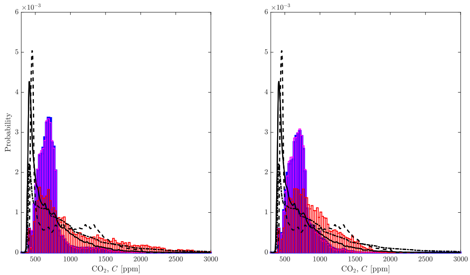
Figure 1: Histograms of the \text{CO}_2 concentrations within the simulated classroom using the weather and \text{PM}_{2.5} data from Leeds: the left-hand pane shows the histograms of the modelled data from the Modern construction classroom and the right-hand pane those from the Victorian ear classroom; both panes include black curves illustrating the PDFs from the measured data (the solid curve marks data reported within Burrige et al. [29], the dashed curve that reported by Vouriot et al. [30], and the dashed-dotted line marks data from the SAMHE Project [65]). blue histograms illustrate the baseline cases, the magenta histograms mark the HEPA cases, and red the HEPA Adjusted cases.
