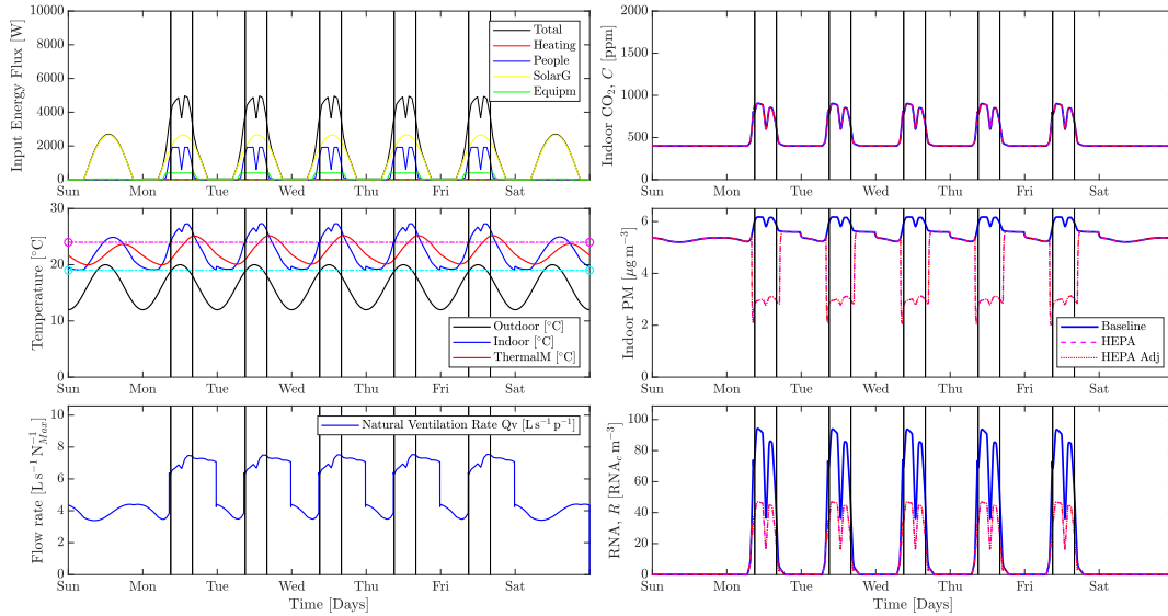
Figure 4: Simulation of summer-like conditions.
