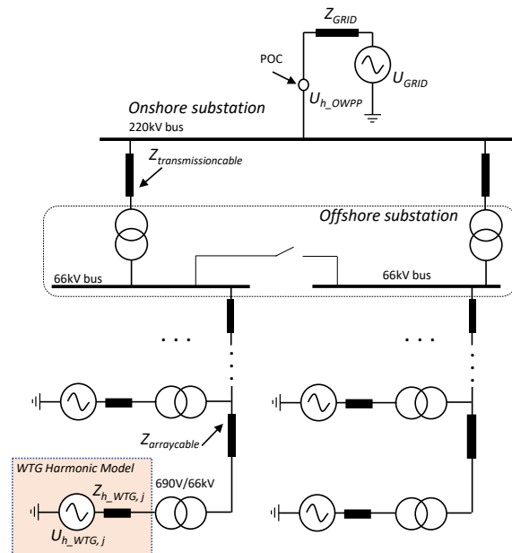
Fig. 12. An example model for the harmonic study of OWPPs.
