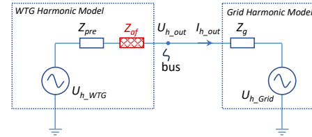
Fig. 14. WTG harmonic model with an active filter.
