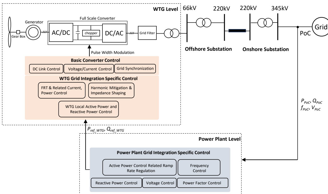
Fig. 9. Control strategies of wind turbine plants.
