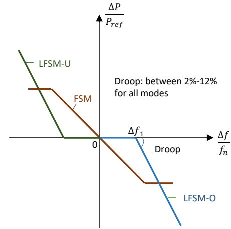
Power- frequency response curve in ENSTO –E RfG
