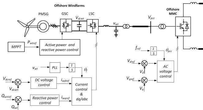
Fig. 21. Control diagrams of WTG and VSC-HVDC for offshore wind power plant transmission.
