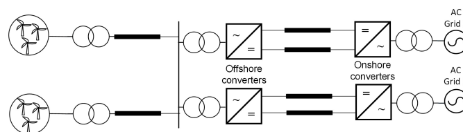
Fig. 16. Parallel connection of HVDC links for OWPP connection.
