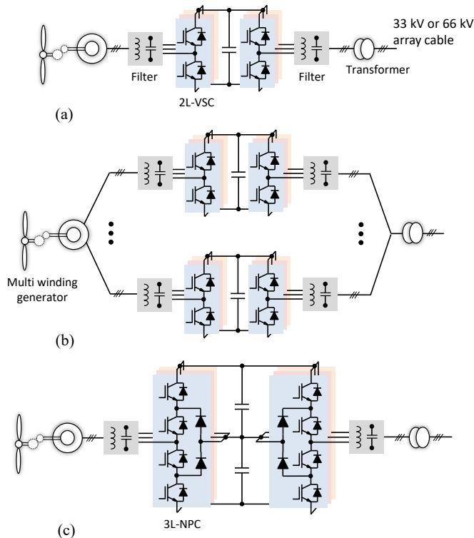
Fig. 8. Offshore wind power converter topologies: (a) two-level back-to-back converter, (b) parallel-connected two-level back-to-back converter, and (c) three-level NPC back-to-back converter.
