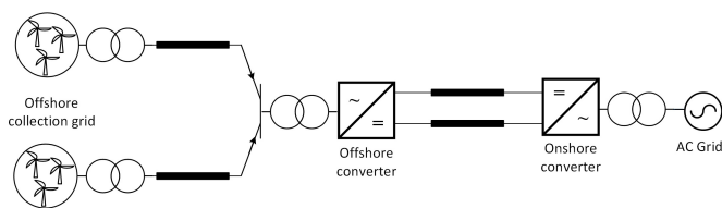
Fig. 15. Typical point-to-point HVDC link for OWPP connection.
