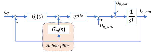
Fig. 13. Diagram of the grid-side wind power converter control with an active filter.
