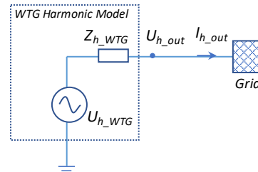
Fig. 7. Harmonic model of wind turbines.
