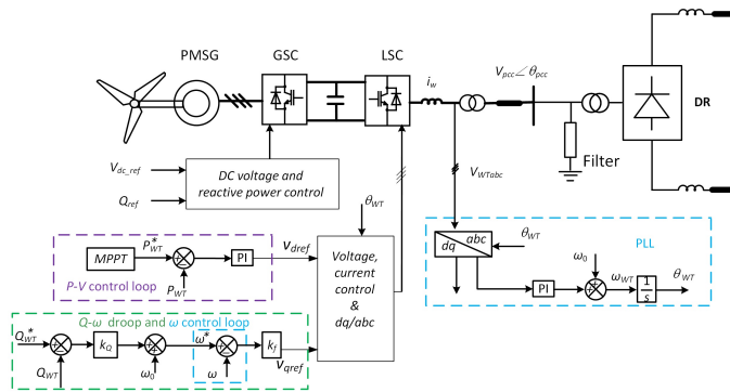
Fig. 22. Distributed PLL control for DR-HVDC-connected OWPPs [66].
