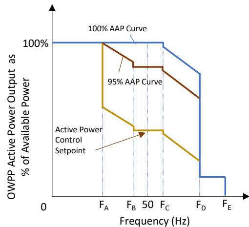
Power- frequency response curve in EirGrid
