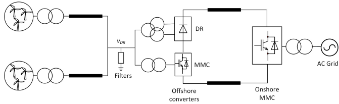
Fig. 19. Configuration of series-connected DR-HVDC and VSC-based HVDC.
