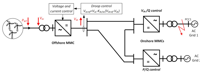
Fig. 23. Onshore fault ride-through Vdc-Vac droop control [131].
