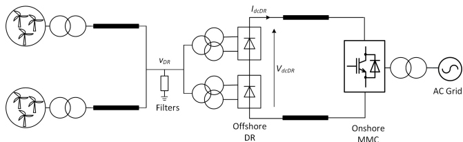
Fig. 18. Configuration of using DR-HVDC for connecting large OWPPs.
