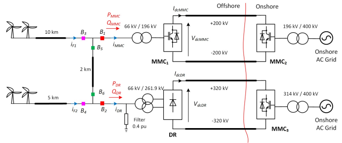
Fig. 20. Hybrid converter station of parallel-connected DR-HVDC and MMC-HVDC systems [92].
