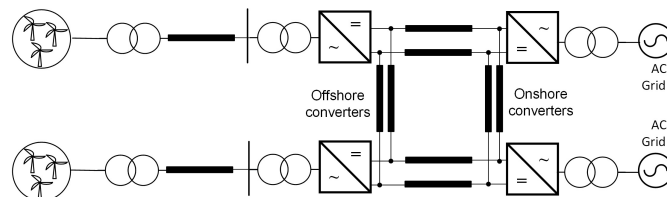
Fig. 17. A four-terminal MTDC system for connecting two large OWPPs.
