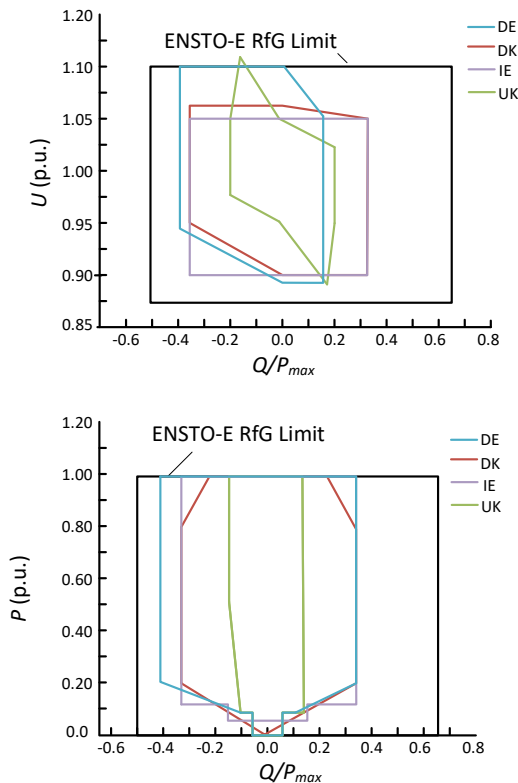
Fig. 4. U-Q and P-Q capability requirement comparison.
