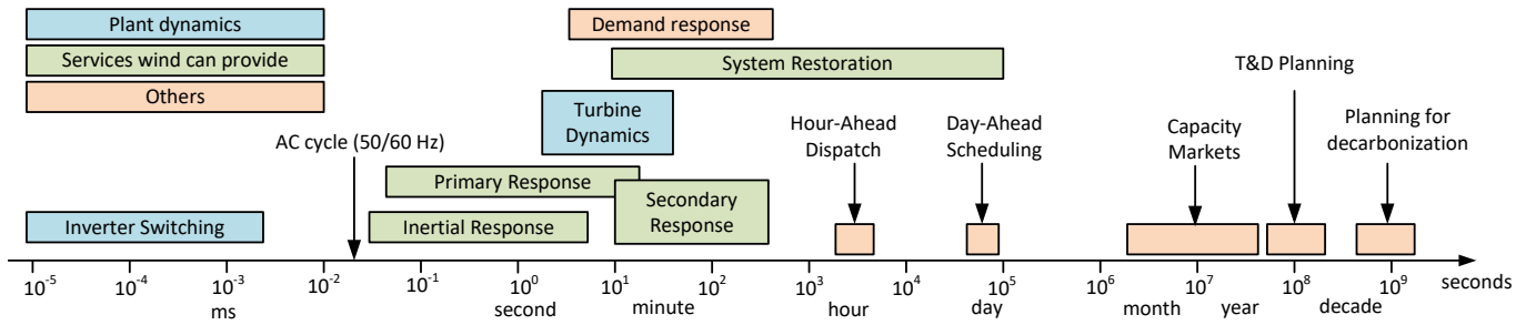
Fig. 10. Ancillary services that wind power plants can provide in different timescales (green) overlaid with inverter and turbine dynamics (blue) and other grid components (orange).
