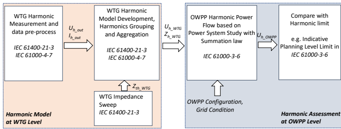
Fig. 11. OWPP harmonic evaluation procedure.
