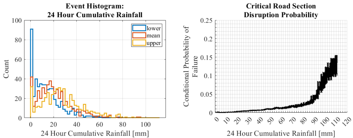
Figure 24 - Histogram of mean and lower and upper 95% confidence bounds for 24 hour cumulative predictions associated with the 506 disruption events (left). Empirical Disruption/Conditional Probability Curve for 24 hour cumulative rainfall (right).
