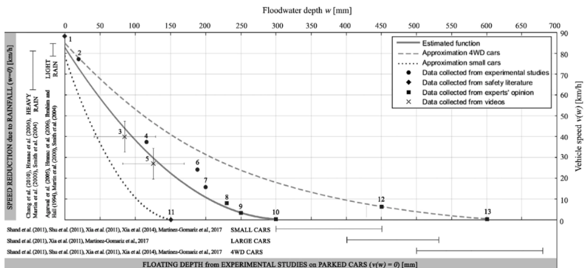
Figure 7 – Depth-disruption function relating flood depth on a road with vehicle speed (Pregmolato et al. , 2017a) ((Creative Commons Attribution 4.0 Licence)
