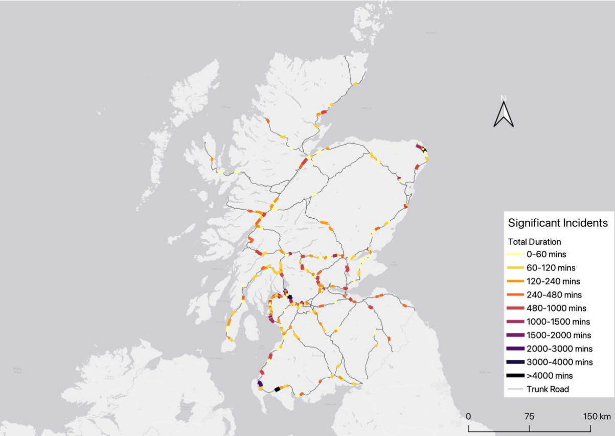
Figure 25 - Recorded flooding incidents by duration
