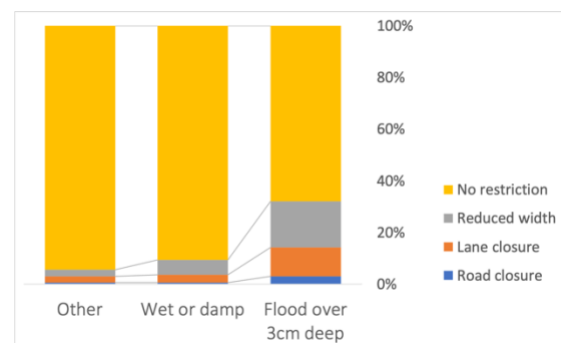
Proportion of Flooding Incidents Categorised by Flood Depth
