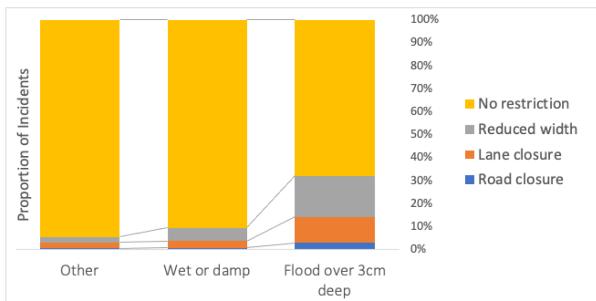
Figure 18 – Proportion of incidents (2014-2021) which resulted in different levels of functionality loss for a given flood depth
