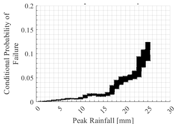
Variation in the Probability of Flooding Disruption with Peak Rainfall
