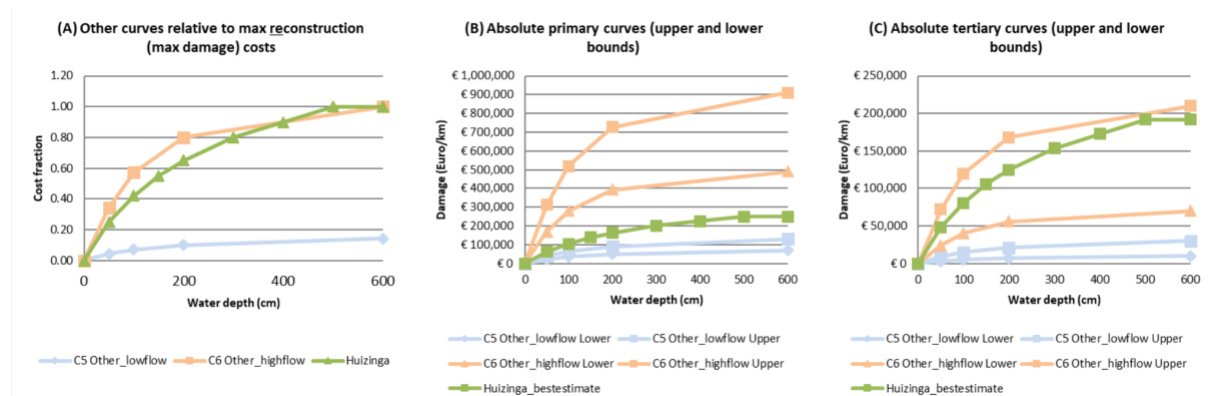
Figure 9 – Vulnerability functions (relative loss and absolute cost) non-trunk roads under low and high-flow conditions (van Ginkel et al. , 2021). (Creative Commons Attribution 4.0 Licence)
