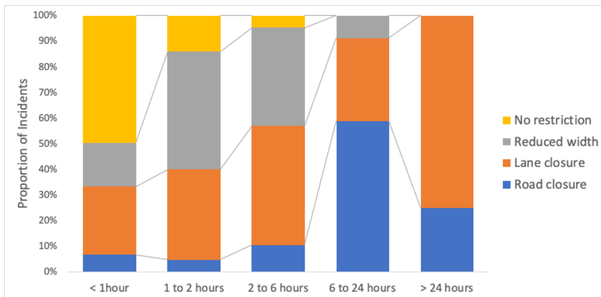
Figure 19 – Proportion of incidents (2014-2021) which resulted in different levels of functionality loss for a given duration of flood incident
