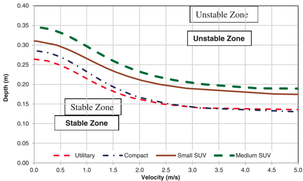
Figure 10 – Stability thresholds by vehicle type (Bocanegra and Francés, 2021). (Creative Commons Attribution Licence)
