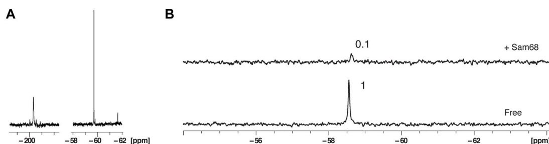
FIGURE 5 Effect of 2'-OCF 3 labelling on 19 F NMR signal sensitivity and protein binding in the presence of nuclear extract. (A) 1D NMR spectra at 303K of fluorinated 2'-F-RNA at position A20 at a concentration of 200 μM (left) and fluorinated 2'-OCF 3 -RNA at position A20 at a concentration of 100 μM (right). The total NMR measurement time per spectrum was 29 min (1,024 scans). (B) 1D NMR spectra at 303K of the 2'-OCF 3 -RNA in the presence of 40% nuclear extract before and after addition of Sam68 at a RNA:protein ratio of 1:2. The total NMR measurement time per spectrum was 7 min (256 scans).
