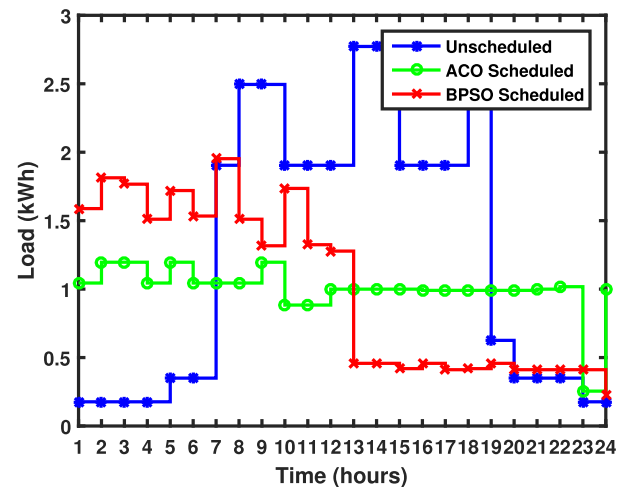
FIGURE 4. Energy consumption.
