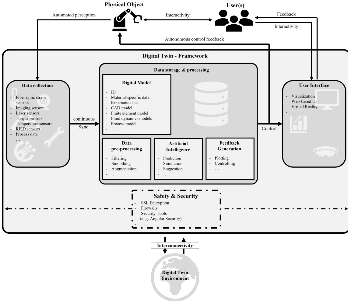
Figure 2: Typical Digital Twin framework in conventional application domains. The physical object is monitored using sensors, a continuously updated digital representation is stored using a database, simulations based on Artificial Intelligence are performed and corresponding feedback is provided to the physical world.
