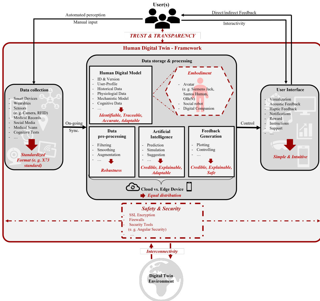
Figure 8: General Human Digital Twin-Framework that extends the conventional Digital Twin framework with the elaborated human factors and considerations – denoted in cursive letters.
