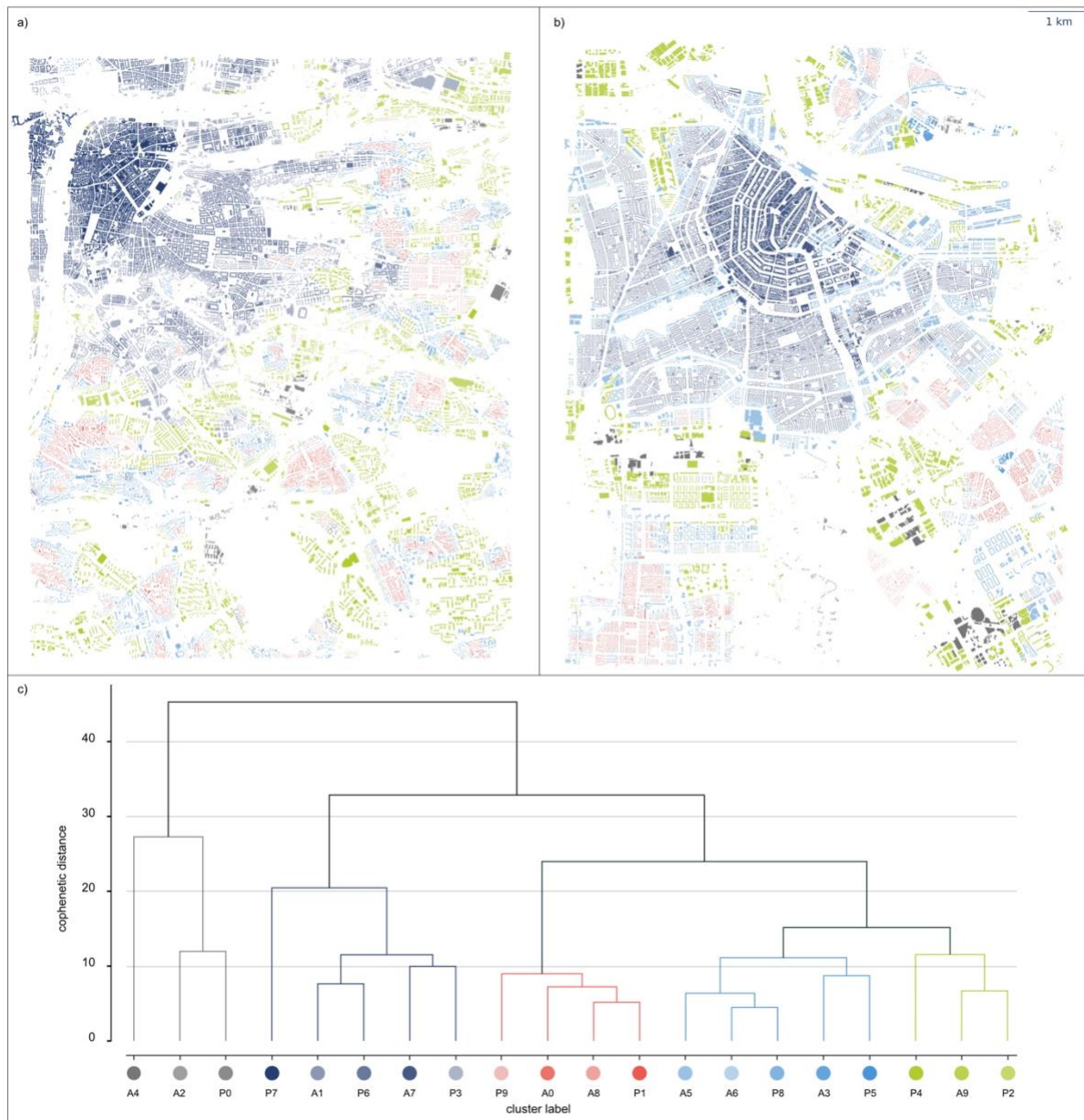
Figure 4: Spatial distribution of different branches of the combined dendrogram in central Prague (a) and central Amsterdam (b) accompanied by the dendrogram representing the results of Ward's hierarchical
