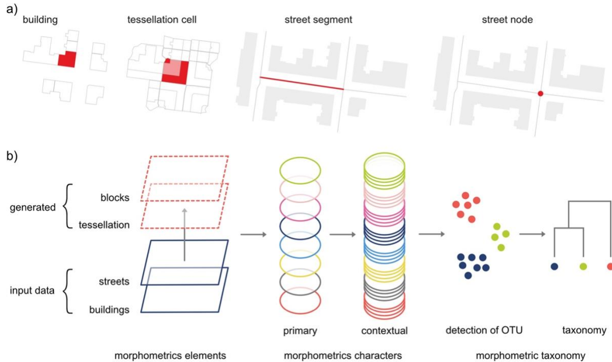
Figure 1: a) Fundamental morphometric elements: building footprint , tessellation cell (derived from building footprints) and street (segment and node from centrelines). b) Diagram illustrating the workflow of the proposed method. From input data (buildings, streets) are derived generated elements (tessellation, blocks). All elements are used to measure primary morphometric characters. Each of them is then represented as 4 contextual characters that are used as an input of the cluster analysis. Finally, resulting classes are organised in a taxonomy.
