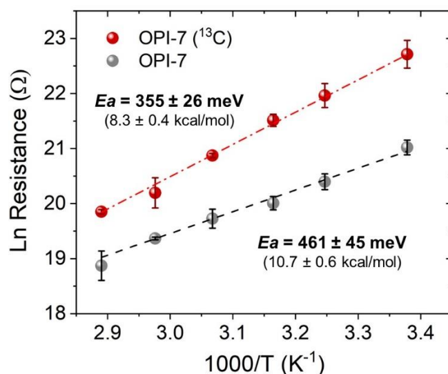
Figure 4. Arrhenius plot for OPI-7 and ^{13}\text{C} -labeled OPI-7 . The activation energies were obtained from the slope of linear fits. Each point corresponds to the average of the low bias resistance in several locations of different samples. Error bars represent standard errors on the mean.
