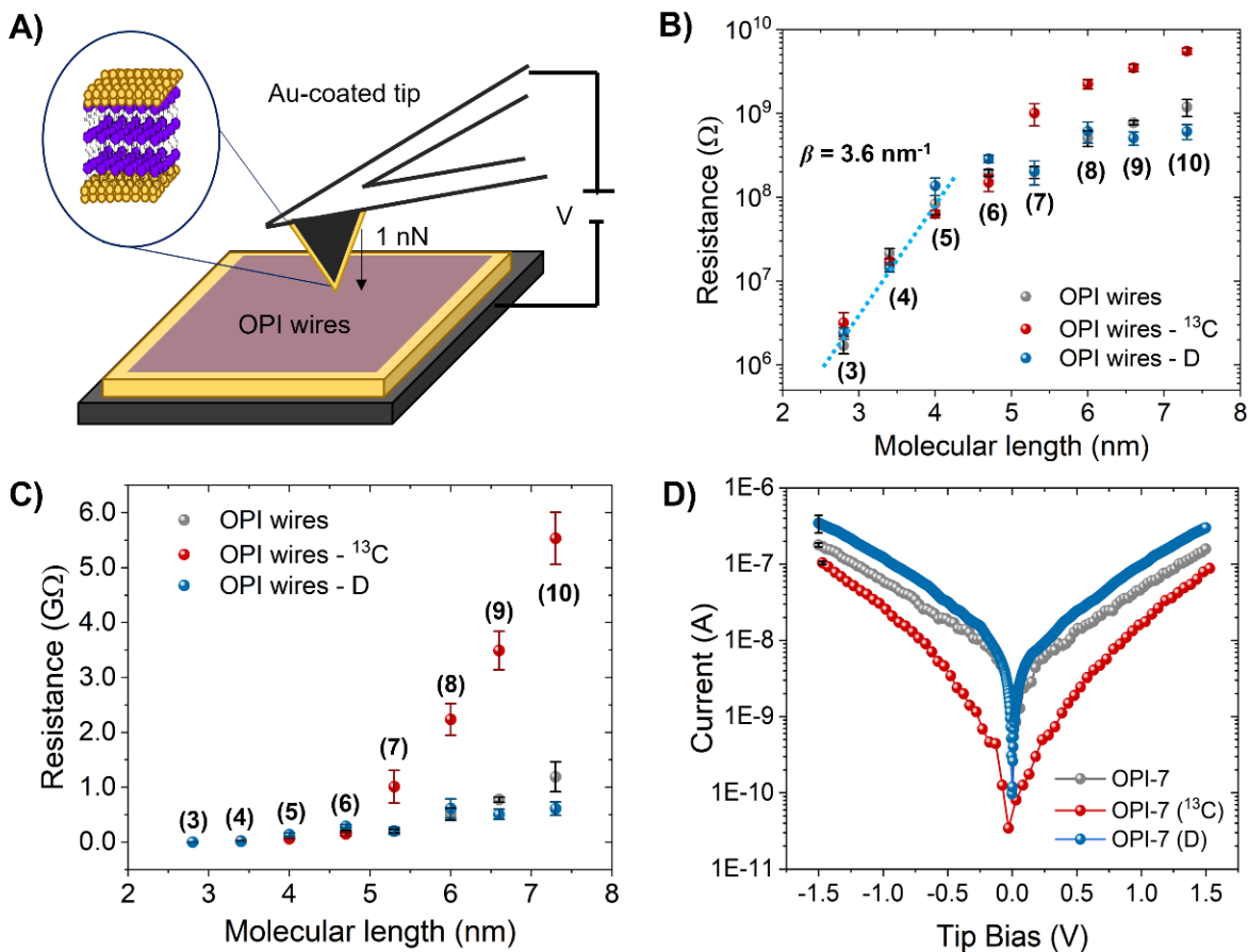
Figure 3. (A) Representation of a molecular junction formed using conducting probe atomic force microscopy (CP-AFM). (B) and (C) Semilog and linear plots of low bias resistance versus molecular length for unlabeled and labeled OPI wires. Each data point is the average of resistances extracted from 800 I - V traces within \pm 0.15 V. Error bars represent standard error. D) Semilog plot of the average current from 250 I - V traces within \pm 1.5 V for the three isotopologues of OPI-7. Error bars represent the standard errors.
