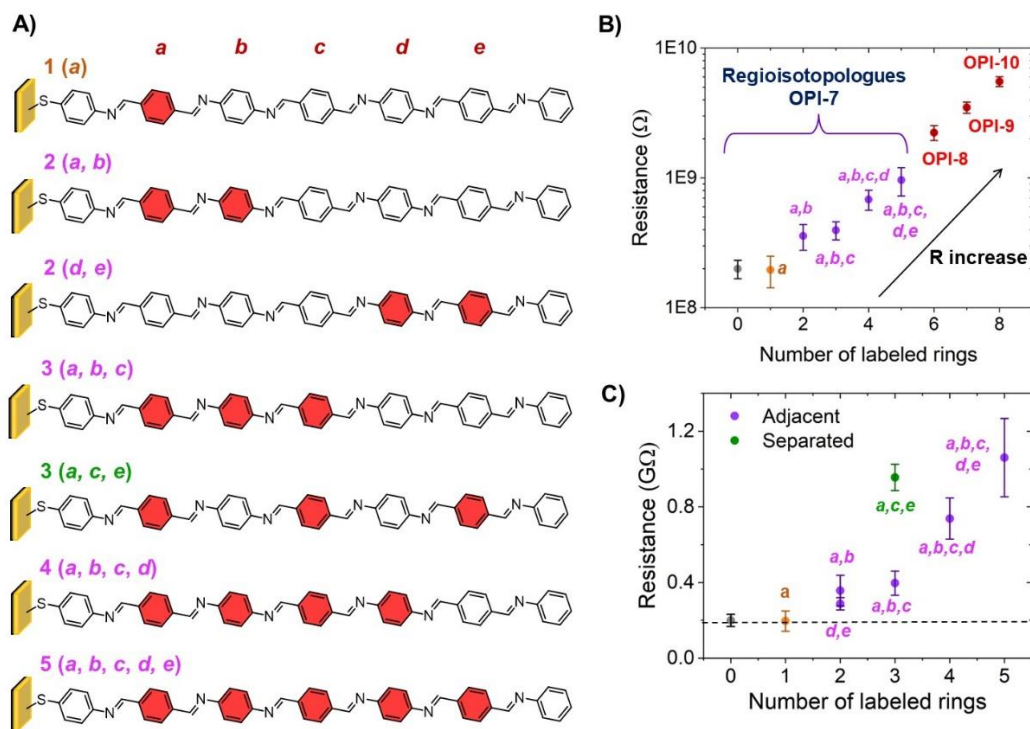
Figure 5. (A) Molecular structures of OPI-7 isotopologues with adjacent (e.g. 3a,b,c ) and separated (e.g., 3a,c,e ) ^{13}\text{C} -labeled rings. (B) Semilog plot of resistance vs number of adjacent labeled rings for OPI wires with n \geq 7 . (C) Linear plot of resistance vs number of adjacent or separated labeled rings for OPI-7 isotopologues. Panel (C) shows data from panel (B) and a new data point for 3a,c,e . Purple data points correspond to structures with adjacent labeled rings. The green data point corresponds to a structure where the labeled rings are separated by unlabeled rings as shown in (A). Error bars represent standard errors and the horizontal black dashed line indicates the resistance of the unlabeled OPI-7 wire.
