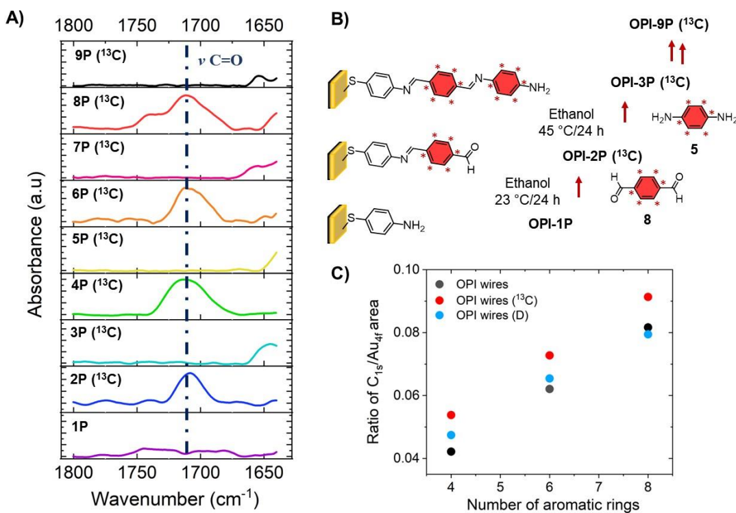
Figure 2. Stepwise characterization of ^{13}\text{C} -labeled OPI wires. (A) RAIRS spectra for OPI- n\text{P} ( n = 1-9 ) where P denotes precursor indicating that wires are not capped with terminal phenyl rings. (B) Scheme of the imine click reaction using monomers 5 and 8 to grow the target molecular wires. (C) Plot of the ratio of \text{C}_{1s}/\text{Au}_{4f} peak areas (285.0 vs. 84.0 eV) from XPS analyses showing similar carbon content for the three isotopologues with the same number of aromatic rings and indicating comparable surface coverage.
