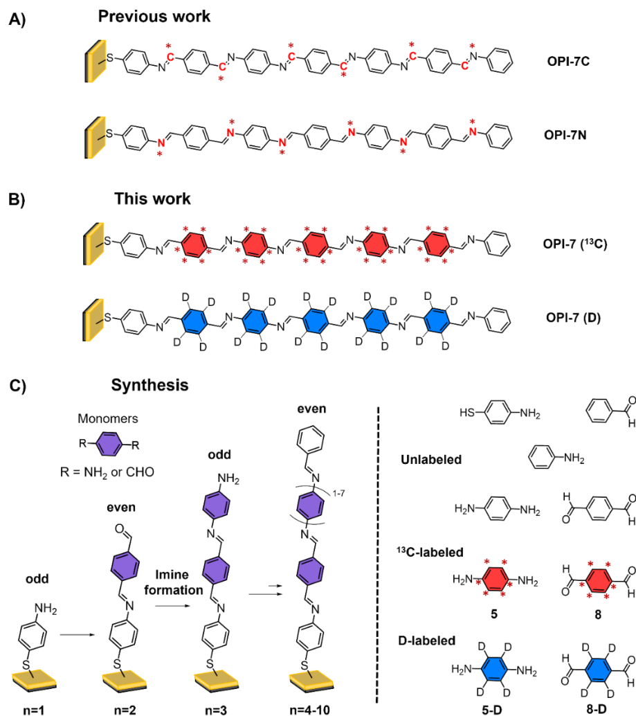
Figure 1. Chemical structures of example oligophenylene imine wires with seven phenylene rings ( OPI-7 ) where (A) the imine groups are labeled with ^{13}\text{C} or ^{15}\text{N} atoms (*) and (B) the aromatic rings are labeled with ^{13}\text{C} (*) or D atoms. (C) Stepwise synthesis of OPI wires and chemical structure of monomers used in the synthesis. Purple colored rings indicate the ^{13}\text{C} or D-labeled units in the wires and n is the number of rings in the oligomer.
