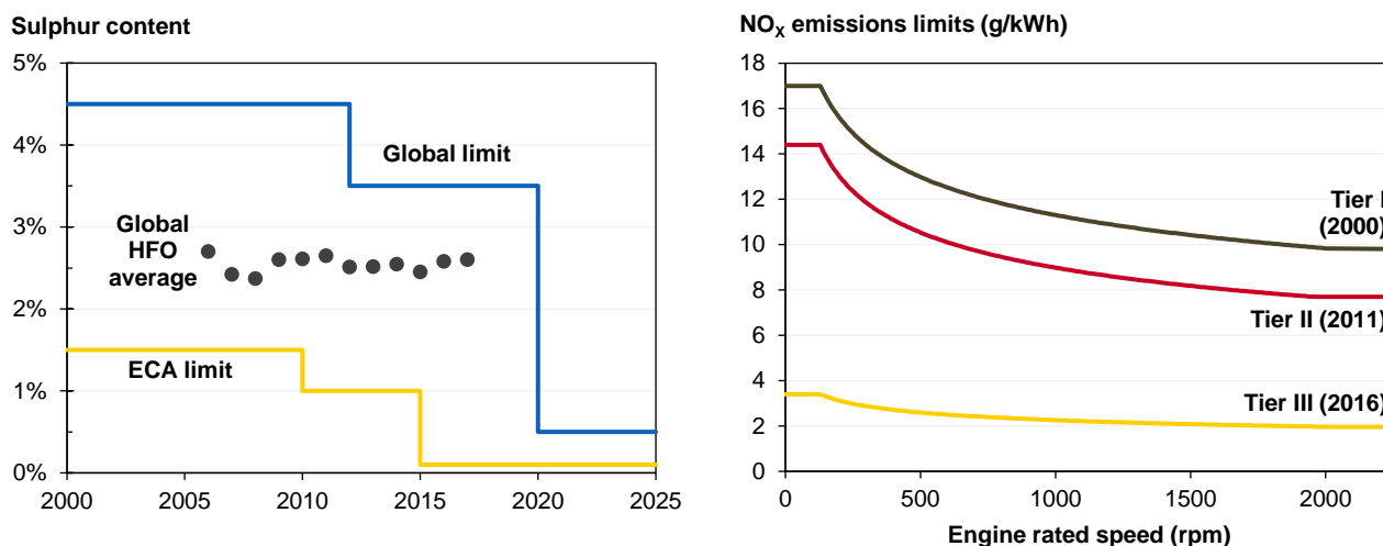
170 Figure 5: Sulphur and nitrogen oxides (NO x ) regulations for shipping fuels. In the left panel, lines show the MARPOL Annex VI limits for open seas and in emissions control areas (ECAs); points show the global average in HFO fuel [3, 17, 32]. In the right panel, lines show the limits as a function of engine speed for open seas (Tier II) and control areas (Tier III) [48].
