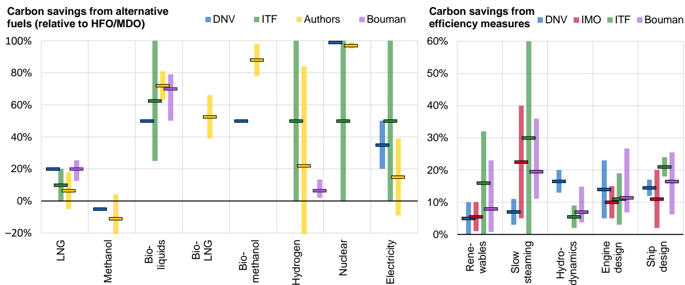
725 Figure 12. Ranges of GHG emissions reductions via the use of alternative fuels (left panel), and from incorporating various efficiency measures (right panel). Alternative fuels are presented relative to the use of conventional fossil liquid fuels, HFO and MDO. Light bars represent the range from each study (1 st /3 rd quartile from Bouman, min/max otherwise), and dark horizontal bars represent the median. Data from [20, 108, 176].
