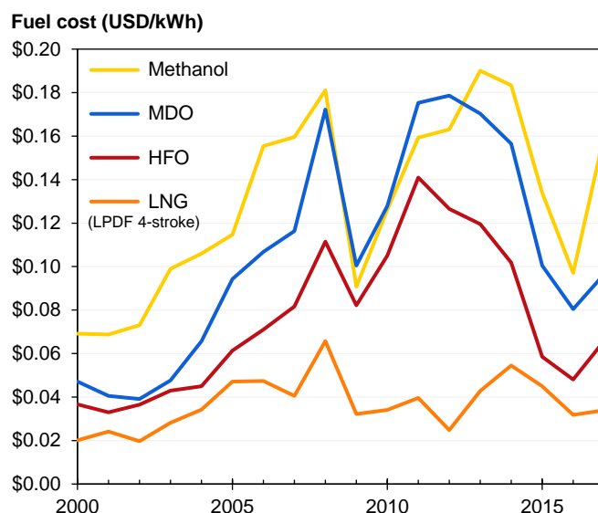
Figure 7: Average fuel costs for each year for different fuels per kWh of engine output. LPDF 4-stroke = low pressure dual fuel 4 stroke run on LNG. Average fuel costs per tonne from [14, 75-81] are converted to engine output using standard engine efficiencies.
