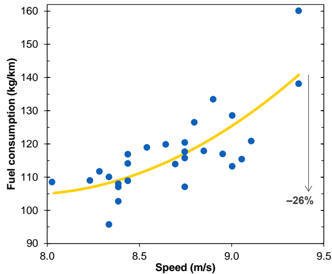
Figure 10: Fuel consumption of sea vessels versus average speed. Data from [140].
