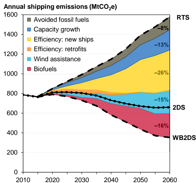
Figure 14. IEA pathway to reduce global shipping emissions by 50% by 2050, highlighting the trajectories anticipated in their scenarios: Reference Technology Scenario, two Degree scenario (2DS) and well below two degree scenario (WB2DS). The contribution from the major efficiency and fuel change measures in 2060 are shown inset to the right. Data from [57]
