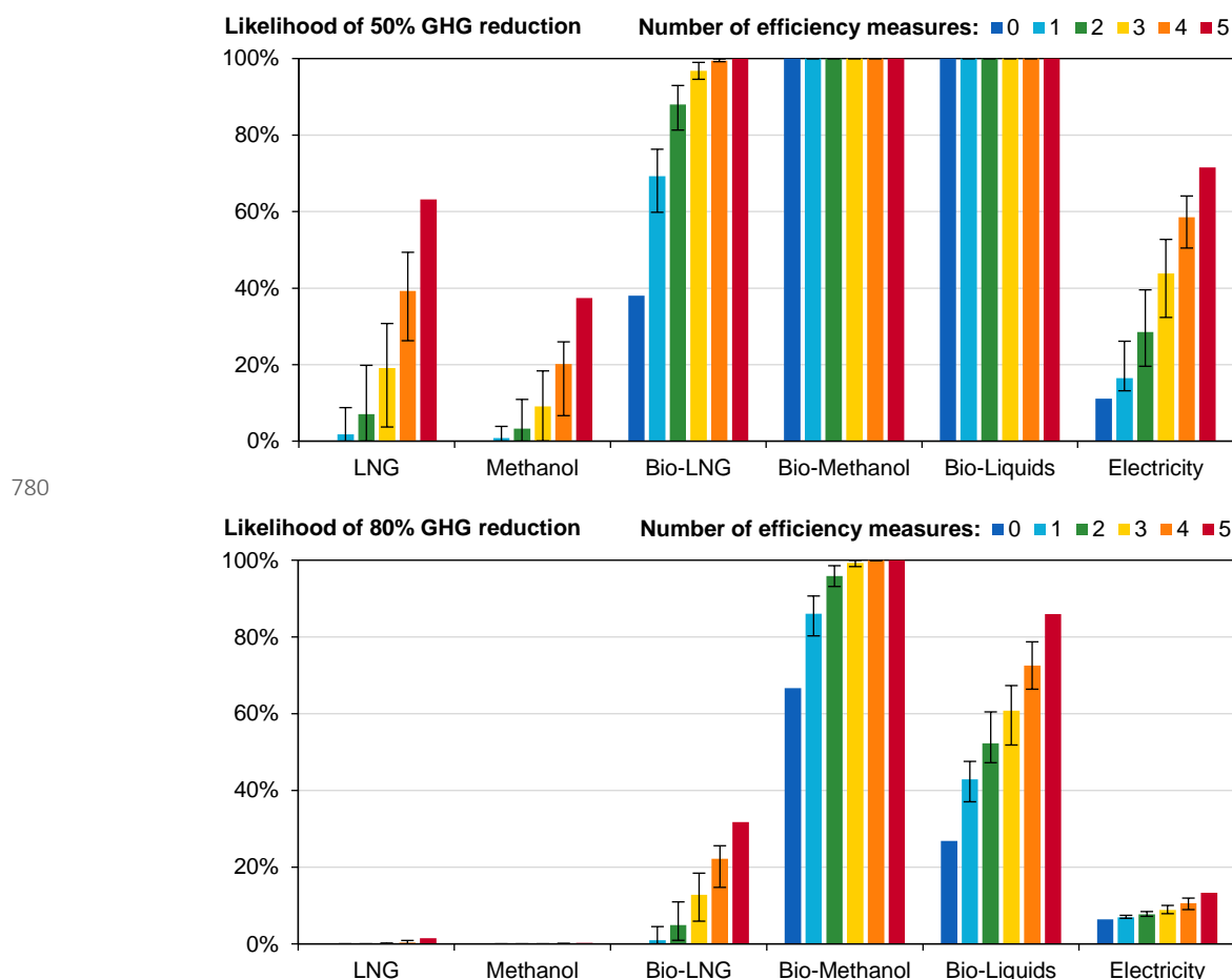
785 Figure 13. Probability of meeting the 50% GHG emission reduction target (top) and a stronger 80% target (bottom) via the use of alternative fuels alongside combinations of 5 different efficiency measures (renewable assisted propulsion, slow steaming, hydrodynamics, engine design and ship design).
