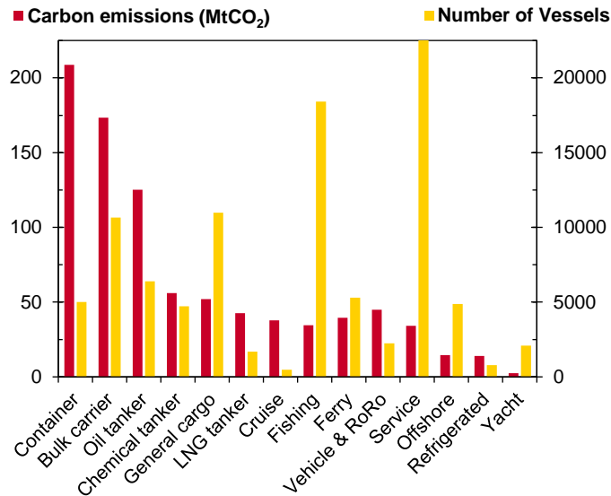
Figure 2. Number of merchant ships and their carbon emissions, by category in 2017. Ferry includes passenger and passenger-RoRo (roll-on roll-off). Data from [30].
