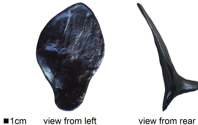
Stegosaurus stenops cervical plate
