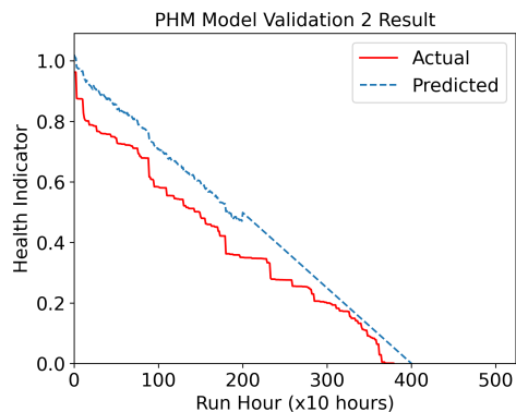
Fig. 6. Validation 2 Result for the trained PHM Model
