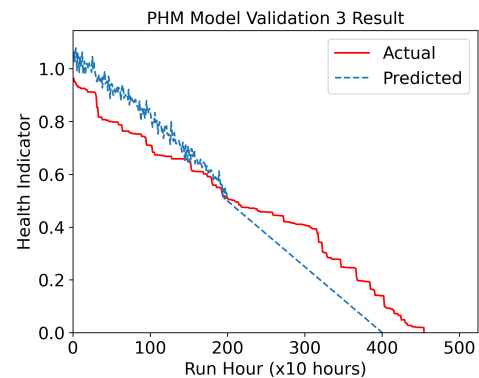
Fig. 7. Validation 3 Result for the trained PHM Model
