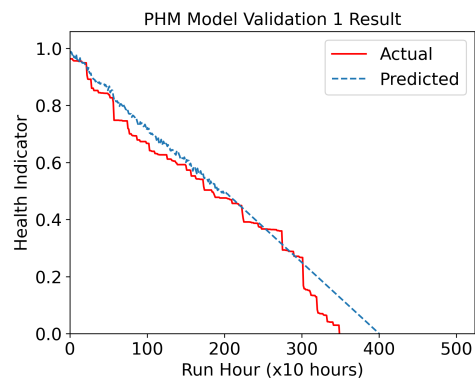
Fig. 5. Validation 1 Result for the trained PHM Model
