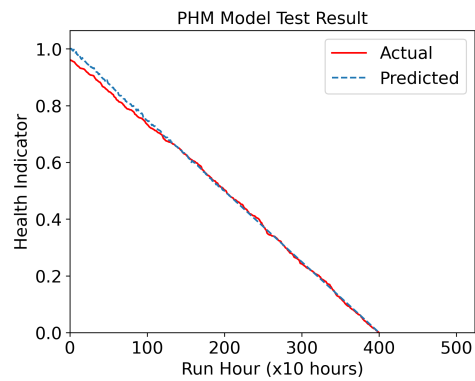
Fig. 4. Test Result for Prediction Model
