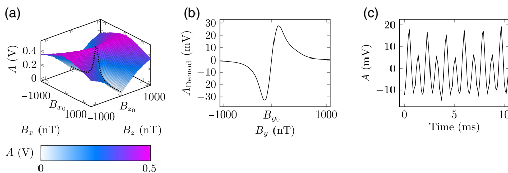
Fig. 6 Experimental signals arising from sensor operation. (a) Transmission of the light through the atomic vapor as a function of the applied field on the x - and z -axes. The narrowest point on this saddle-like landscape indicates the field values necessary to null the residual field. The peak transverse resonance at zero-field is indicated by the black dotted line. (b) The modulated Hanle response, a plot of demodulated voltage as a function of applied field on the y -axis. The slope of the linear region (mV/nT) may be used to convert from demodulated voltage to magnetic field units. (c) The free-running signal measured on the PD with respect to time.
