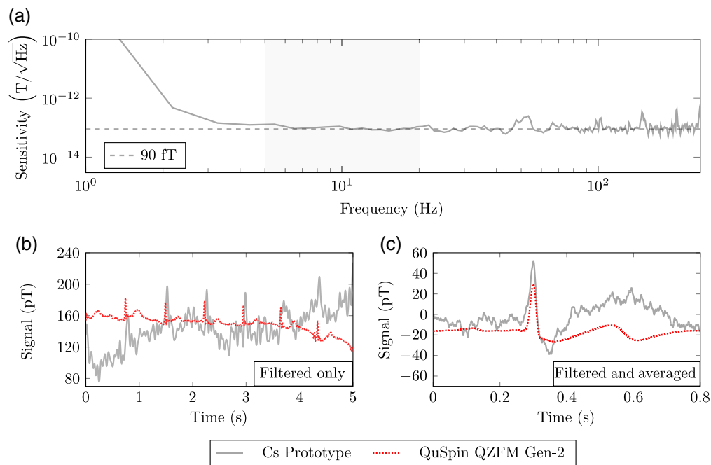
Fig. 9 (a) Measured magnetic noise floor of the sensor. The frequency band used to calculate sensitivity of the sensor is highlighted in gray. The dashed line indicates the geometric mean calculated in the frequency band of interest. This measurement was taken in a five-layer Mu-metal shield (Magnetic Shields Limited). (b), (c) Magnetocardiogram measured simultaneously using the portable cesium prototype sensor and QuSpin QZFM Gen-2 sensor inside an MSR, using a band-pass filter from 1 to 40 Hz on both responses. (b) Real-time responses of both sensors, without averaging. (c) Both responses averaged across 60 heartbeats.
