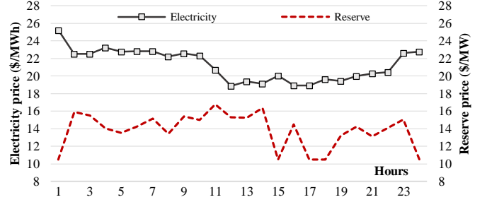
Fig. 10. Prices of electricity and reserve with ICRA at high load
