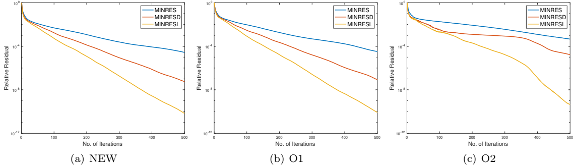
FIG. 6. Residual plots – performance of different preconditioners for one iteration of NEW, O1 and O2 in Test1. Here, MINRES, MINRES D and MINRES L represent that the solver is MINRES without preconditioner, with diagonal preconditioner and with L preconditioner respectively.
