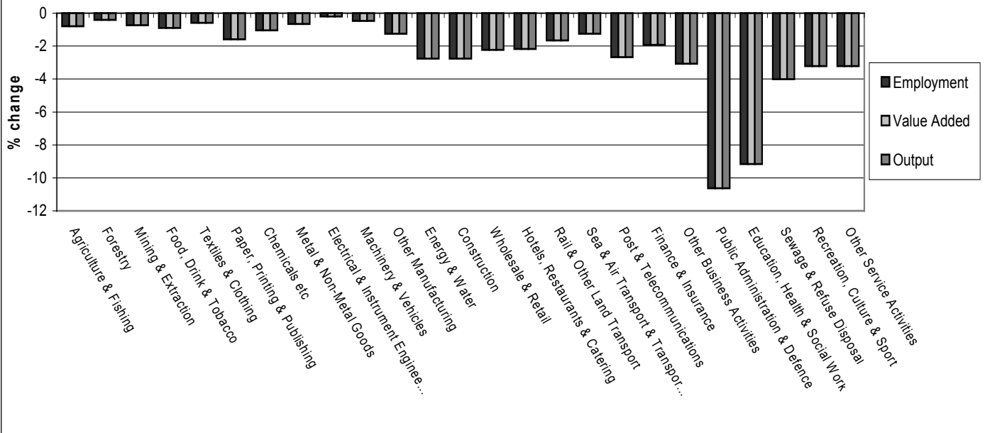
Figure 5 - Long-run sectorally-disaggregated changes in employment, value added and output with Barnett fixed population weights equilibrium
