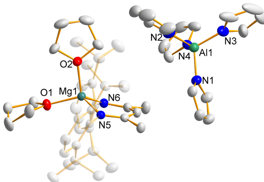
Fig. 4 Ion pair structure of [(\text{DIPFP})\text{Mg-2THF}]^+ [\text{Al}(\text{pyr})_4]^- ( 5 ) with hydrogen atoms and minor disordered component of a THF backbone omitted for clarity and with thermal ellipsoids drawn at 50% probability. Selected bond lengths (Å) and angles ( ^\circ ): Al–N, 1.842(2)–1.861(2) av. 1.851; Mg1–N5, 2.024(2); Mg1–N6, 2.006(2); Mg1–O1, 1.991(2); Mg1–O2, 1.987(2); N–Al–N, 107.5(1)–111.7(1) av. 109.4; N5–Mg1–N6, 96.31(7); O1–Mg1–O2, 99.33(7); N5–Mg1–O1, 120.17(7); N5–Mg1–O2, 112.46(7); N6–Mg1–O1, 113.72(7); N6–Mg1–O2, 115.99(7).
