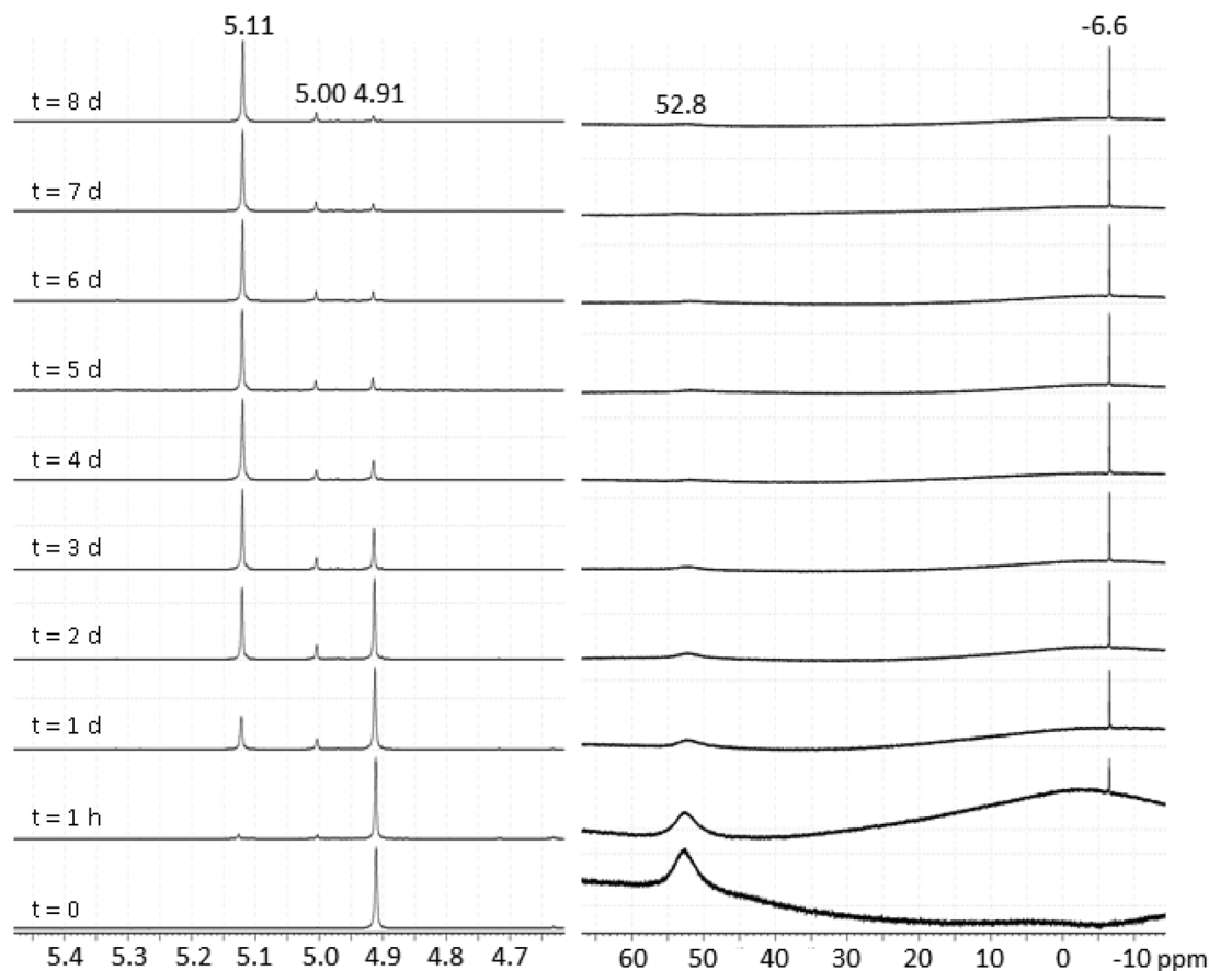
Fig. 2 Section of ^1\text{H} (left) and ^{11}\text{B} NMR spectra (right) of NMR scale reaction of ^{\text{Dipp}}\text{NacNacMgPh} and \text{BPh}_3 in d_8 -THF showing the region diagnostic of the \text{C}_\gamma\text{-H} of the ^{\text{Dipp}}\text{NacNac} species; all values in ppm.
