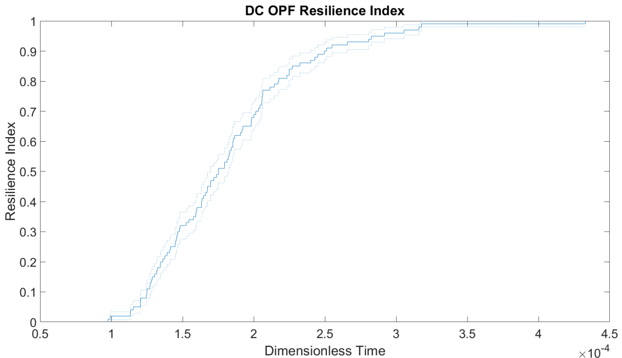
Figure 2: Results for DC-OPF simulation
