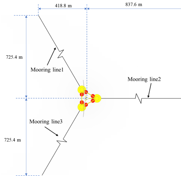
Figure 2. Diagram of mooring arrangement.
