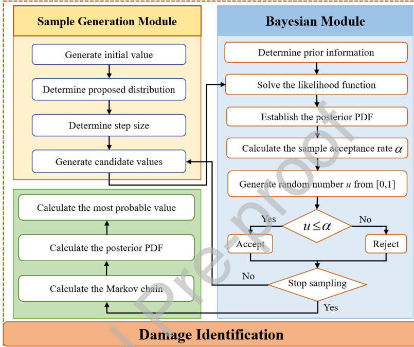
Figure 5. The flowchart of the damage identification
