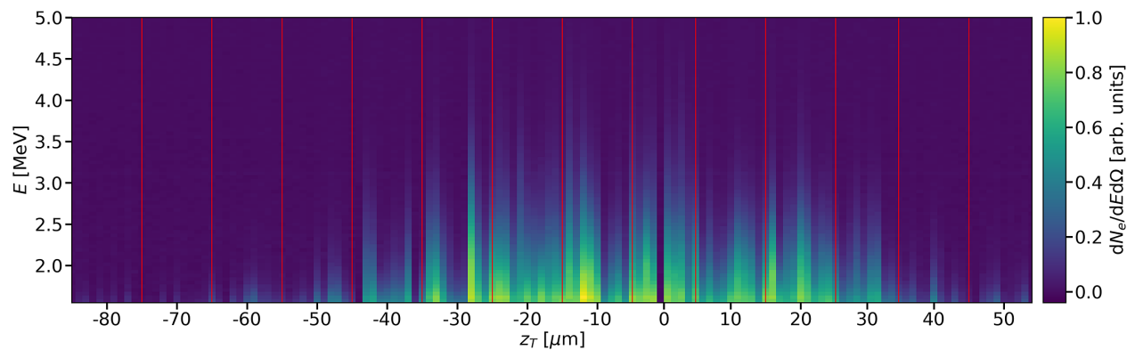
Figure 9. Waterfall plot of the normalized forward propagating hot electron spectrum from 50 \mu\text{m} Kapton tape, integrated over the electron spectrometer acceptance angle of 35 \mu\text{Sr} , as the tape-drive position was scanned through the laser focus. Negative values of z correspond to arrival of the laser pulse at the tape surface before the laser has reached best focus. Each vertical strip corresponds to the single-shot electron spectrum at the recorded z position, which was incremented in steps of 10 \mu\text{m} between bursts of 10 shots. Vertical (red) lines mark the boundaries of the bursts and the shots within the burst marked z_T = 0 correspond to the shots presented in Figure 10.
