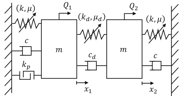
Fig. 1 Representation of the two-mass system with a free-play gap
