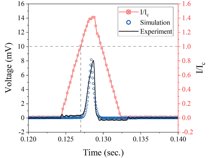
Figure 2. Voltage profile for 8 cm long HTS tape measured experimentally and calculated by FEM simulation against normalized applied current ( I/I_c ).
