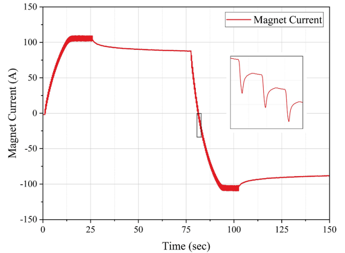
Figure 5. A jointless HTS magnet is charged to its critical current value using a flux pump and the flux pump is switched OFF at time t = 26 s, its current decay can be observed due to self field flux creep at critical state and the current stabilizes at 85 A.
