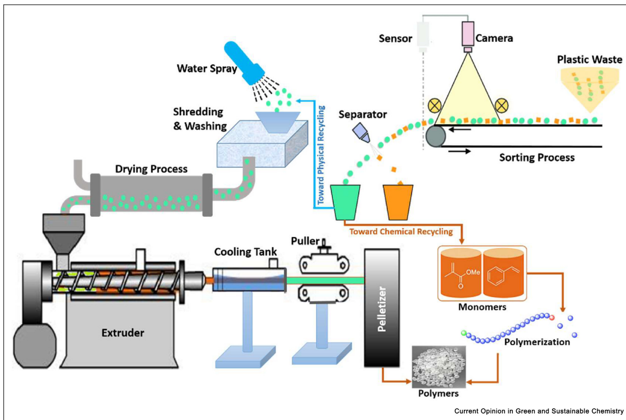
Schematic illustration of plastic waste recycling via mechanical and chemical methods.
