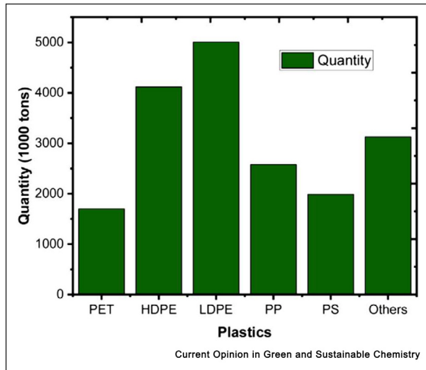
Different types of plastic wastes and their estimated quantities [30].
