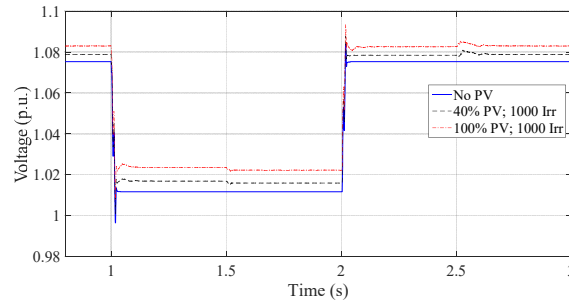
Fig. 10: RMS voltage in phase A at substation for a fault at F2 for different penetration levels of PV with PV distributed near the substation and irradiance of 1000 \text{ W/m}^2
